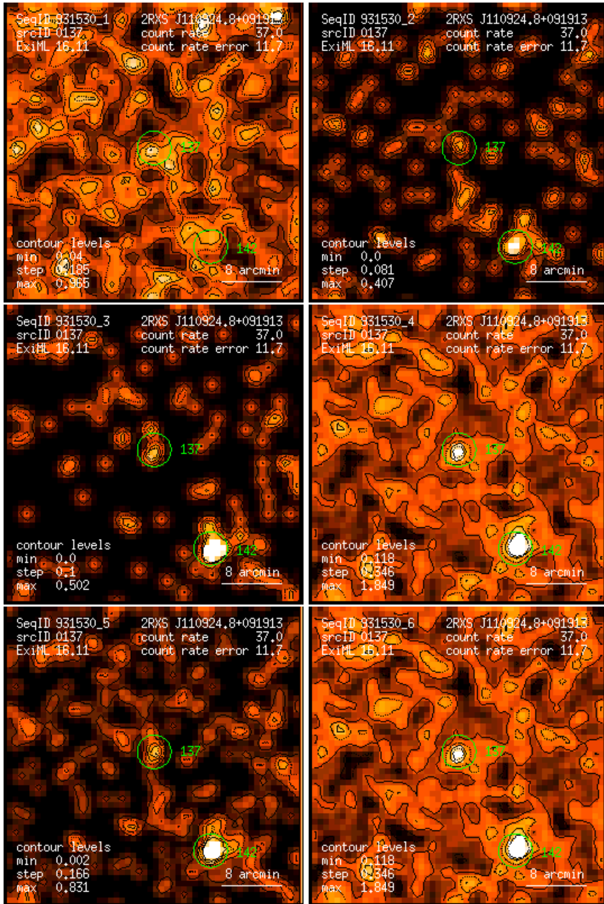
Figure 137: RASS 931530: detection 0137: band rate images, Gaussian filter: (1) PSPC channels 11 – 41, (2) 52 – 90, (3) 91 – 201, (4) 11 – 235, (5) 52 – 201, (6) 11 – 201. Broad band rates in counts/ks. Band rate contour levels in counts/ks/arcmin 2 .
