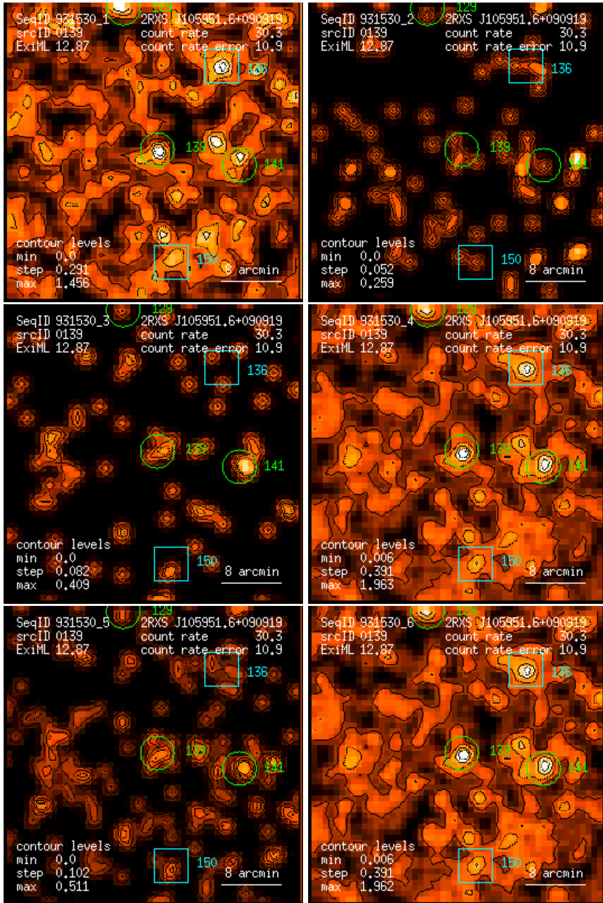
Figure 139: RASS 931530: detection 0139: band rate images, Gaussian filter: (1) PSPC channels 11 – 41, (2) 52 – 90, (3) 91 – 201, (4) 11 – 235, (5) 52 – 201, (6) 11 – 201. Broad band rates in counts/ks. Band rate contour levels in counts/ks/arcmin 2 .
