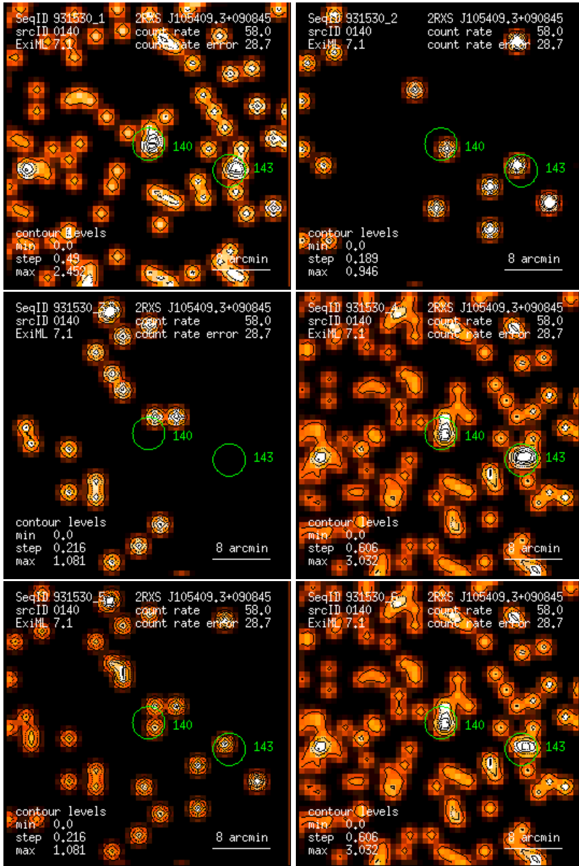
Figure 140: RASS 931530: detection 0140: band rate images, Gaussian filter: (1) PSPC channels 11 – 41, (2) 52 – 90, (3) 91 – 201, (4) 11 – 235, (5) 52 – 201, (6) 11 – 201. Broad band rates in counts/ks. Band rate contour levels in counts/ks/arcmin 2 .
