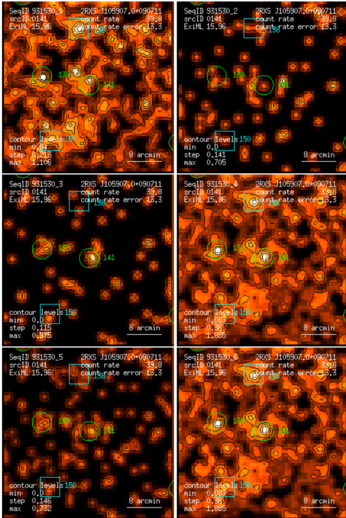
Figure 141: RASS 931530: detection 0141: band rate images, Gaussian filter: (1) PSPC channels 11 – 41, (2) 52 – 90, (3) 91 – 201, (4) 11 – 235, (5) 52 – 201, (6) 11 – 201. Broad band rates in counts/ks. Band rate contour levels in counts/ks/arcmin 2 .
