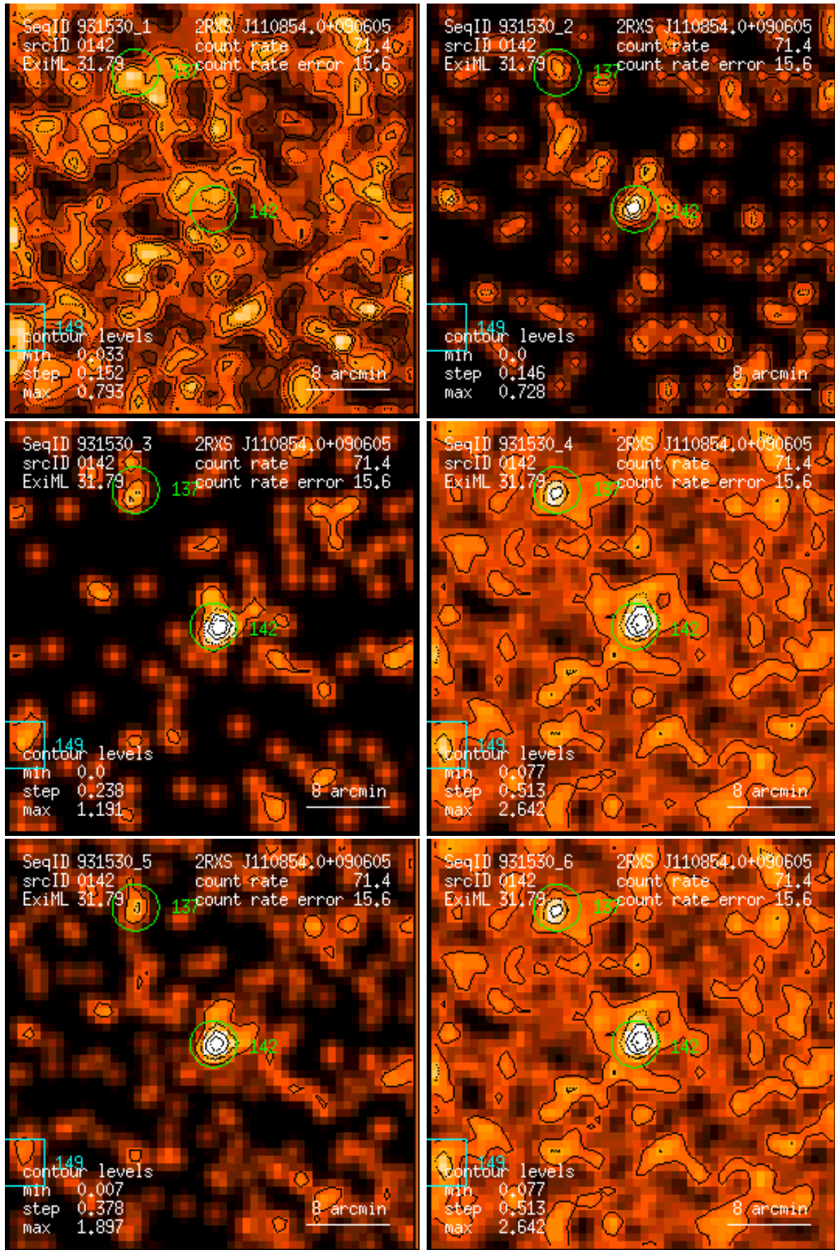
Figure 142: RASS 931530: detection 0142: band rate images, Gaussian filter: (1) PSPC channels 11 – 41, (2) 52 – 90, (3) 91 – 201, (4) 11 – 235, (5) 52 – 201, (6) 11 – 201. Broad band rates in counts/ks. Band rate contour levels in counts/ks/arcmin 2 .
