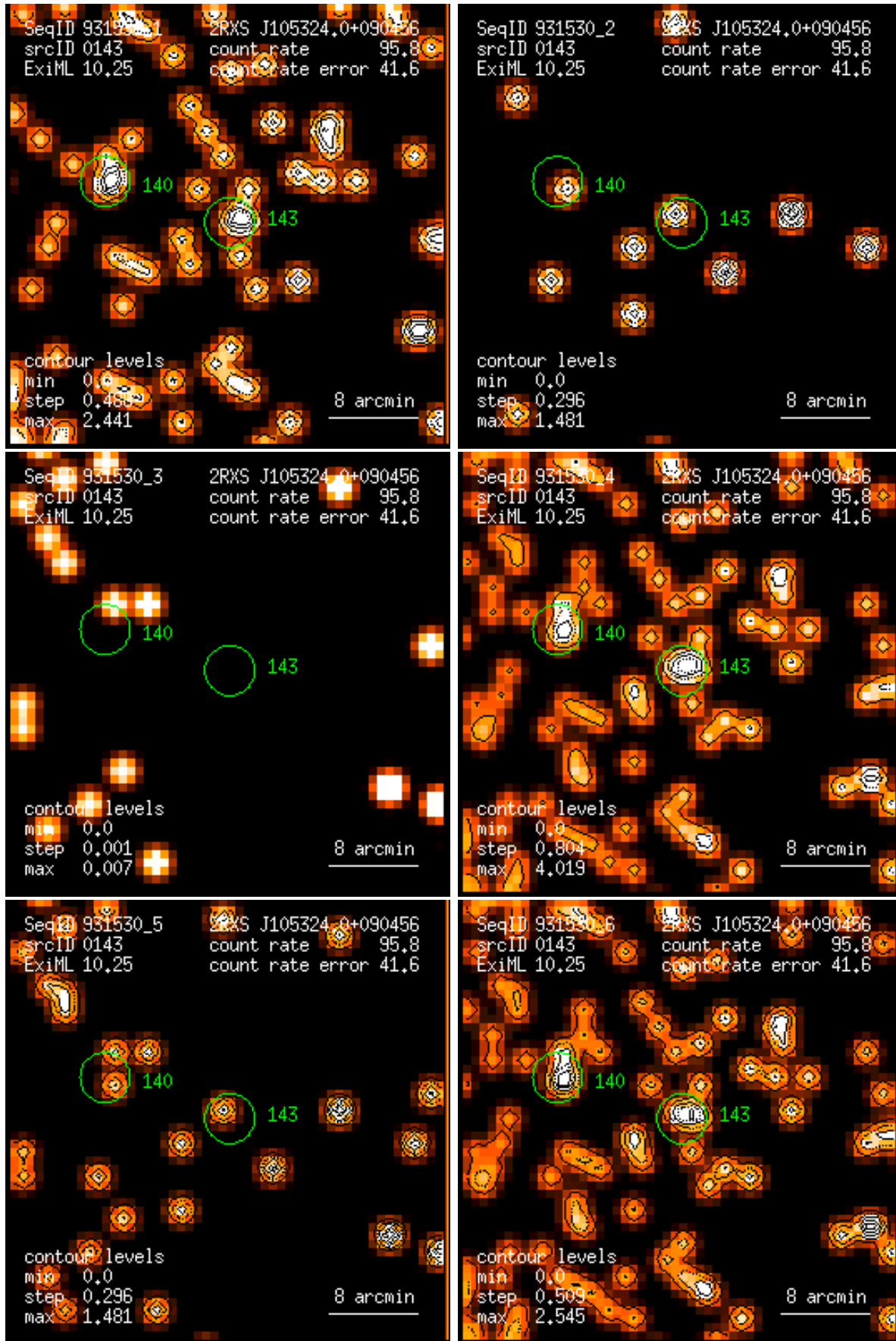
Figure 143: RASS 931530: detection 0143: band rate images, Gaussian filter: (1) PSPC channels 11 – 41, (2) 52 – 90, (3) 91 – 201, (4) 11 – 235, (5) 52 – 201, (6) 11 – 201. Broad band rates in counts/ks. Band rate contour levels in counts/ks/arcmin 2 .
