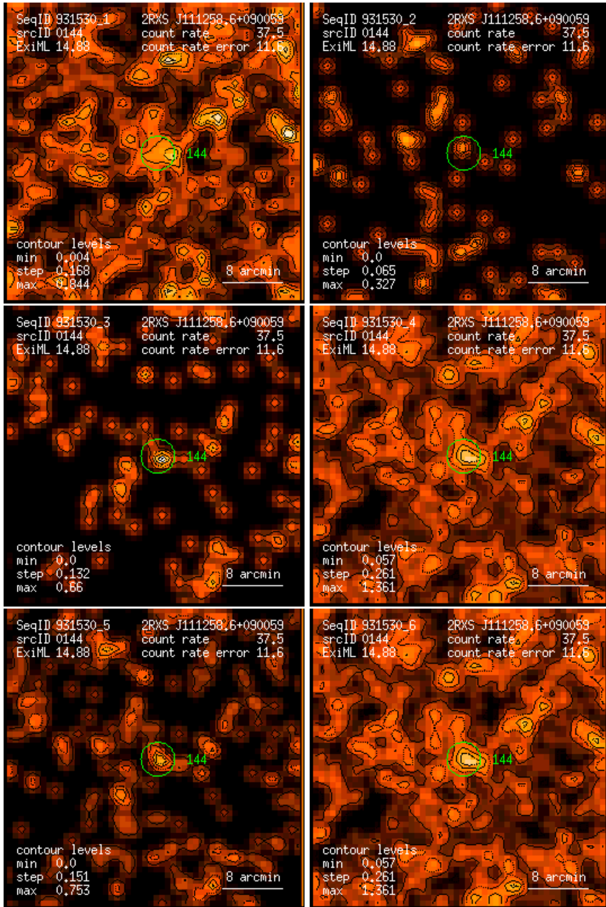
Figure 144: RASS 931530: detection 0144: band rate images, Gaussian filter: (1) PSPC channels 11 – 41, (2) 52 – 90, (3) 91 – 201, (4) 11 – 235, (5) 52 – 201, (6) 11 – 201. Broad band rates in counts/ks. Band rate contour levels in counts/ks/arcmin 2 .
