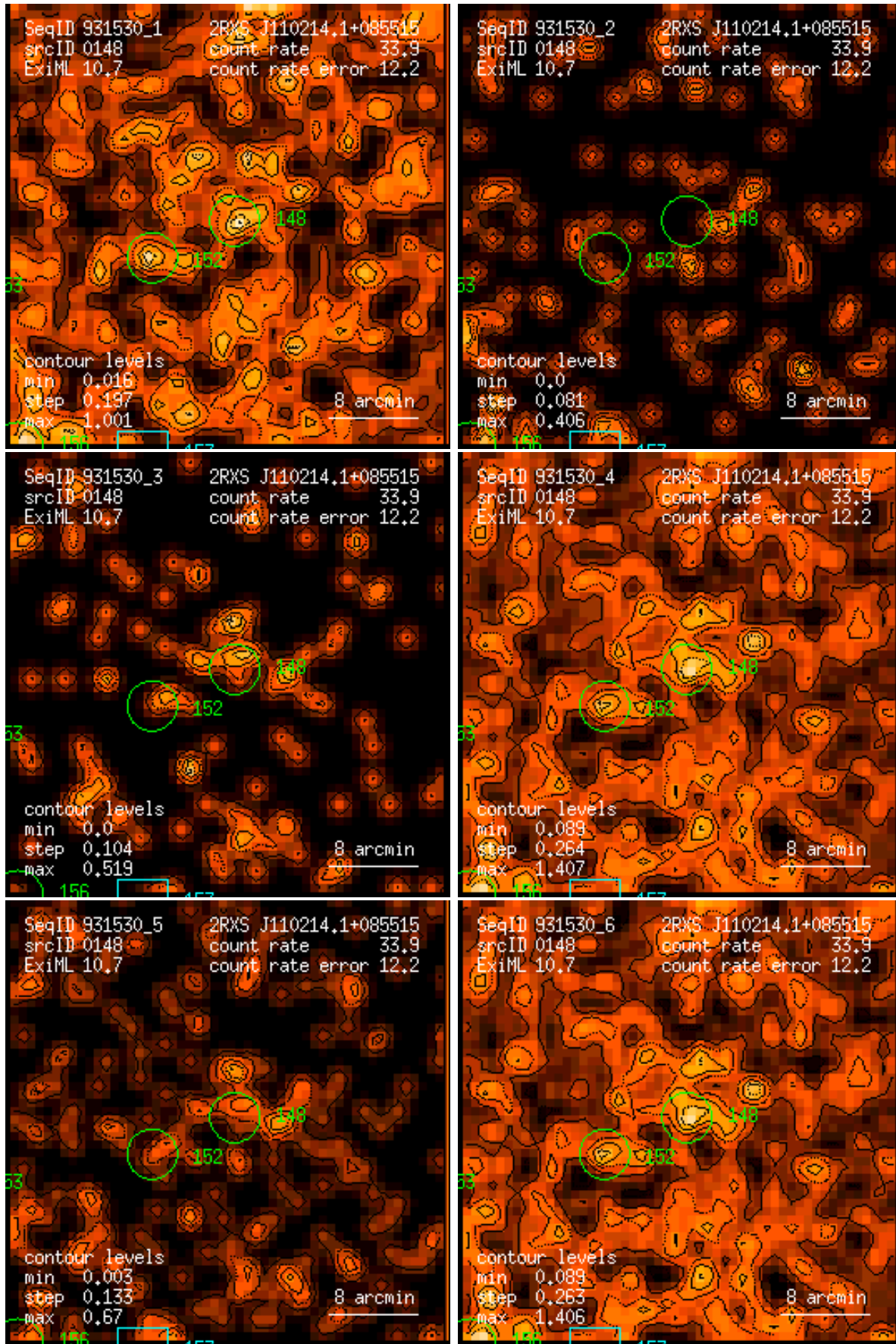
Figure 148: RASS 931530: detection 0148: band rate images, Gaussian filter: (1) PSPC channels 11 – 41, (2) 52 – 90, (3) 91 – 201, (4) 11 – 235, (5) 52 – 201, (6) 11 – 201. Broad band rates in counts/ks. Band rate contour levels in counts/ks/arcmin 2 .
