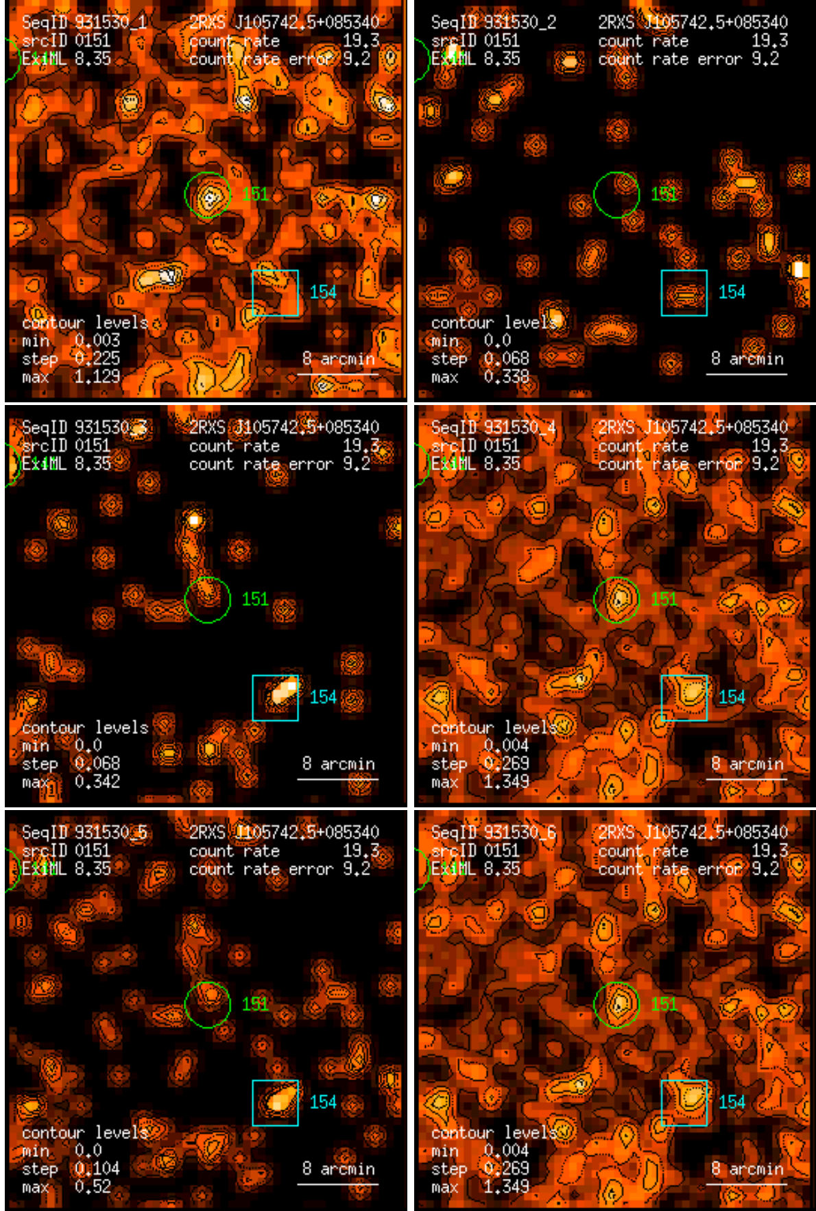
Figure 151: RASS 931530: detection 0151: band rate images, Gaussian filter: (1) PSPC channels 11 – 41, (2) 52 – 90, (3) 91 – 201, (4) 11 – 235, (5) 52 – 201, (6) 11 – 201. Broad band rates in counts/ks. Band rate contour levels in counts/ks/arcmin 2 .
