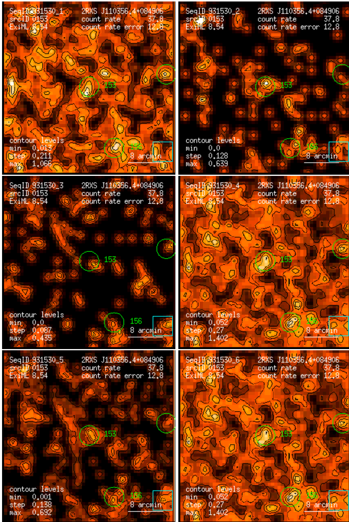
Figure 153: RASS 931530: detection 0153: band rate images, Gaussian filter: (1) PSPC channels 11 – 41, (2) 52 – 90, (3) 91 – 201, (4) 11 – 235, (5) 52 – 201, (6) 11 – 201. Broad band rates in counts/ks. Band rate contour levels in counts/ks/arcmin 2 .
