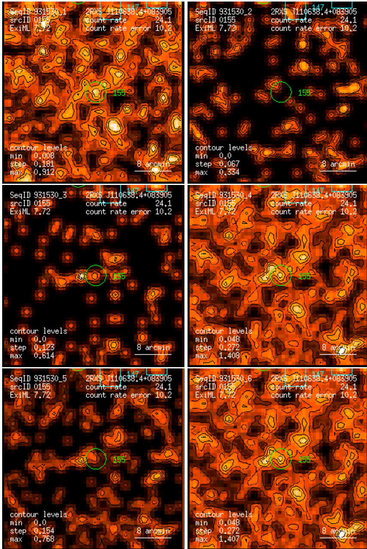
Figure 155: RASS 931530: detection 0155: band rate images, Gaussian filter: (1) PSPC channels 11 – 41, (2) 52 – 90, (3) 91 – 201, (4) 11 – 235, (5) 52 – 201, (6) 11 – 201. Broad band rates in counts/ks. Band rate contour levels in counts/ks/arcmin 2 .
