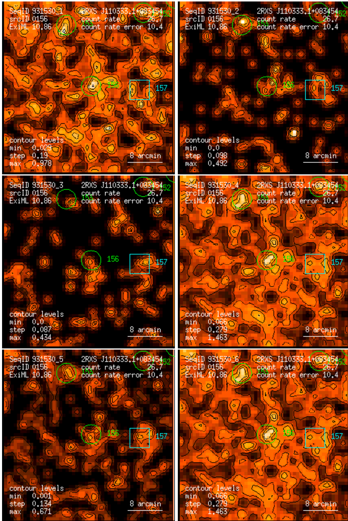
Figure 156: RASS 931530: detection 0156: band rate images, Gaussian filter: (1) PSPC channels 11 – 41, (2) 52 – 90, (3) 91 – 201, (4) 11 – 235, (5) 52 – 201, (6) 11 – 201. Broad band rates in counts/ks. Band rate contour levels in counts/ks/arcmin 2 .
