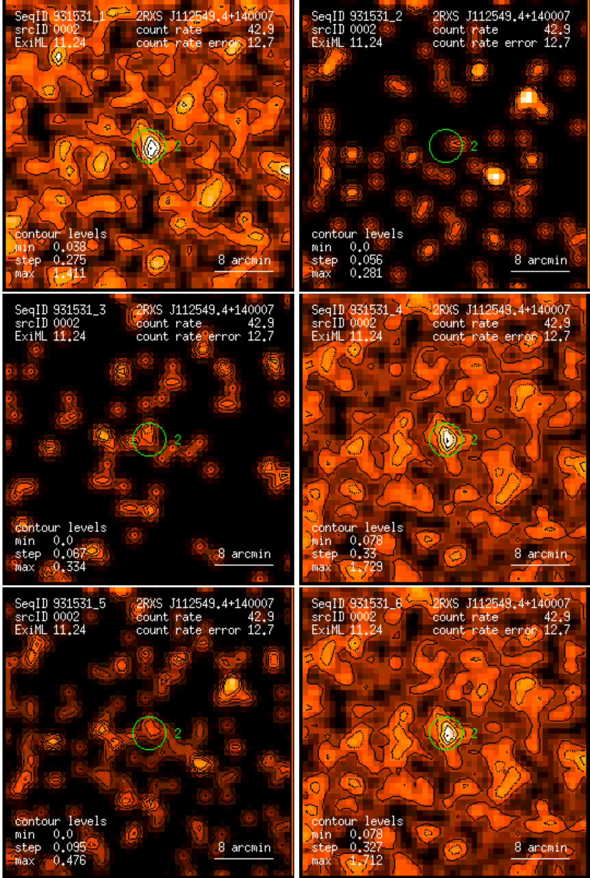
Figure 2: RASS 931531: detection 0002: band rate images, Gaussian filter: (1) PSPC channels 11 – 41, (2) 52 – 90, (3) 91 – 201, (4) 11 – 235, (5) 52 – 201, (6) 11 – 201. Broad band rates in counts/ks. Band rate contour levels in counts/ks/arcmin 2 .
