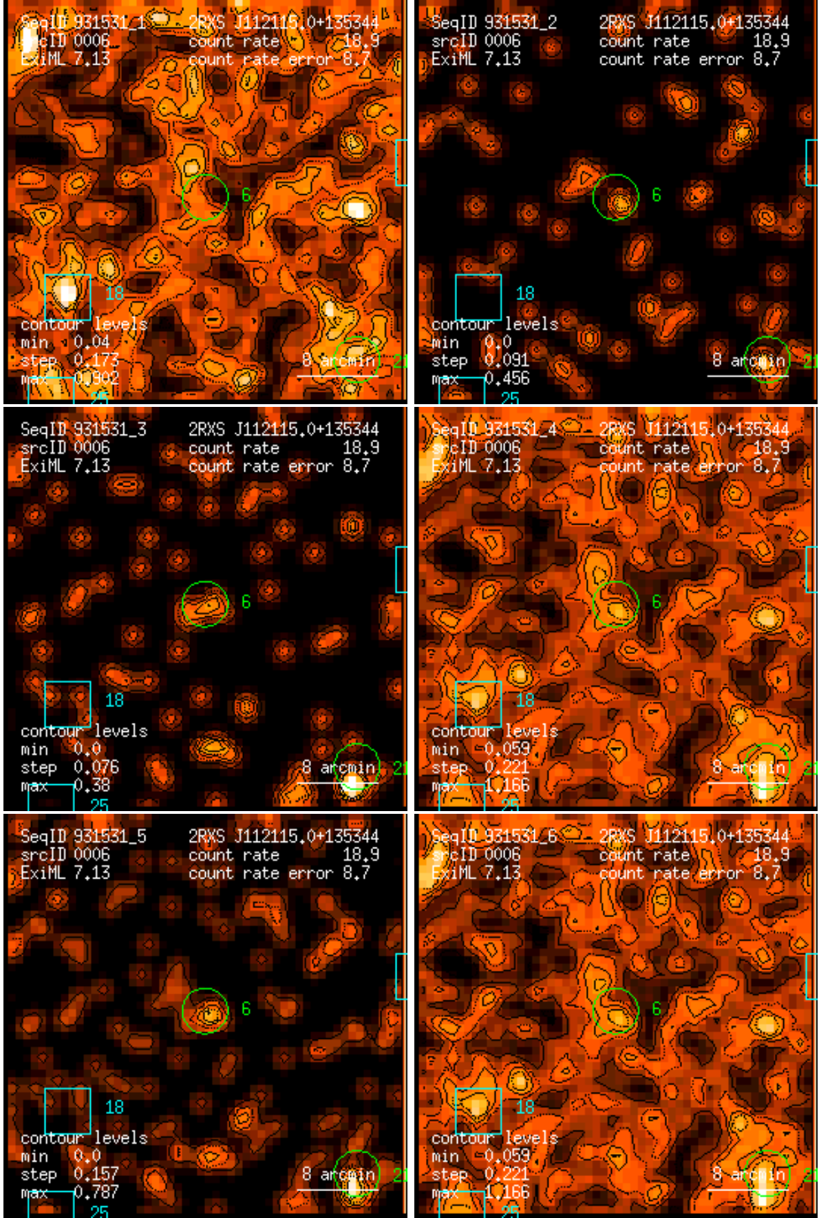
Figure 6: RASS 931531: detection 0006: band rate images, Gaussian filter: (1) PSPC channels 11 – 41, (2) 52 – 90, (3) 91 – 201, (4) 11 – 235, (5) 52 – 201, (6) 11 – 201. Broad band rates in counts/ks. Band rate contour levels in counts/ks/arcmin 2 .
