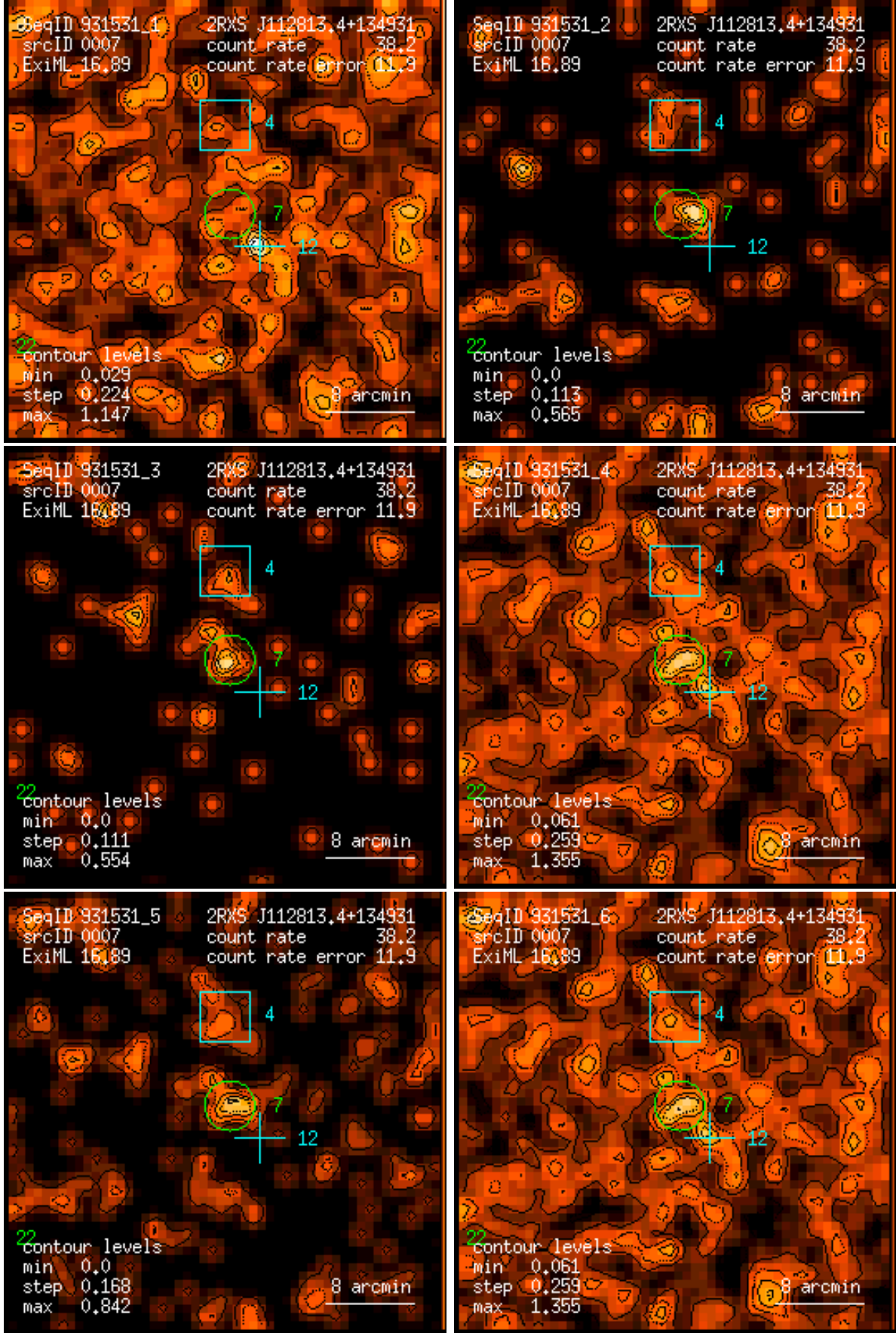
Figure 7: RASS 931531: detection 0007: band rate images, Gaussian filter: (1) PSPC channels 11 – 41, (2) 52 – 90, (3) 91 – 201, (4) 11 – 235, (5) 52 – 201, (6) 11 – 201. Broad band rates in counts/ks. Band rate contour levels in counts/ks/arcmin 2 .
