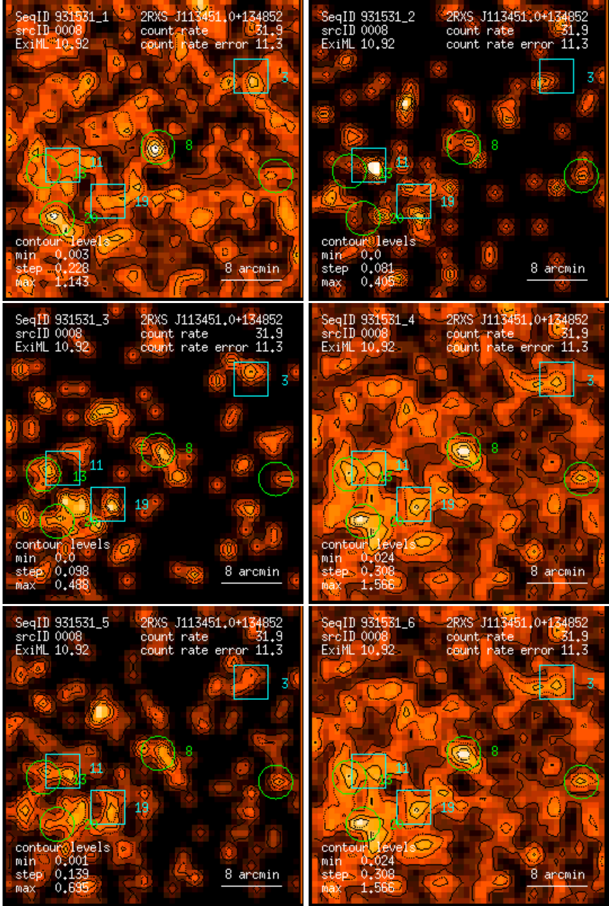
Figure 8: RASS 931531: detection 0008: band rate images, Gaussian filter: (1) PSPC channels 11 – 41, (2) 52 – 90, (3) 91 – 201, (4) 11 – 235, (5) 52 – 201, (6) 11 – 201. Broad band rates in counts/ks. Band rate contour levels in counts/ks/arcmin 2 .
