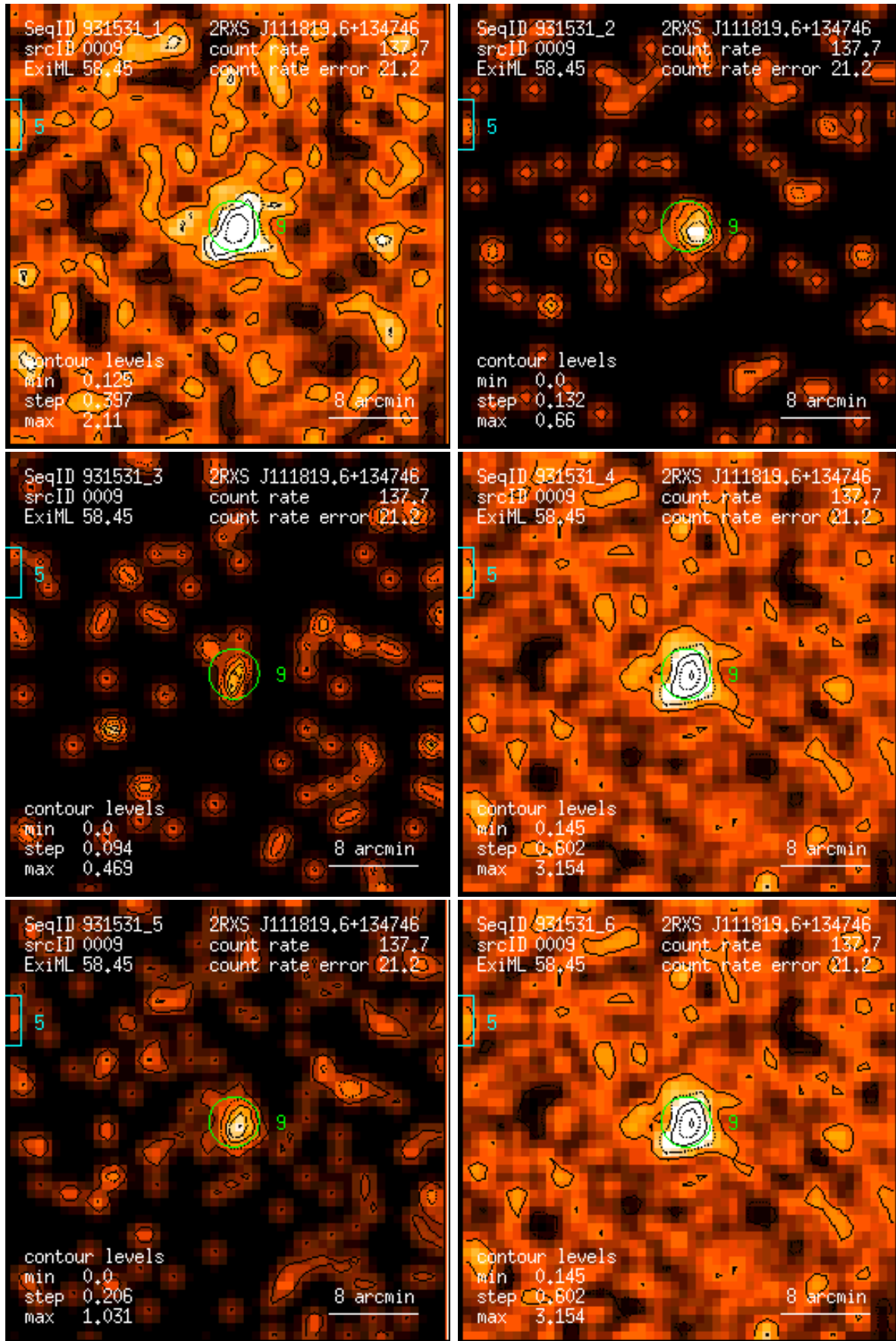
Figure 9: RASS 931531: detection 0009: band rate images, Gaussian filter: (1) PSPC channels 11 – 41, (2) 52 – 90, (3) 91 – 201, (4) 11 – 235, (5) 52 – 201, (6) 11 – 201. Broad band rates in counts/ks. Band rate contour levels in counts/ks/arcmin 2 .
