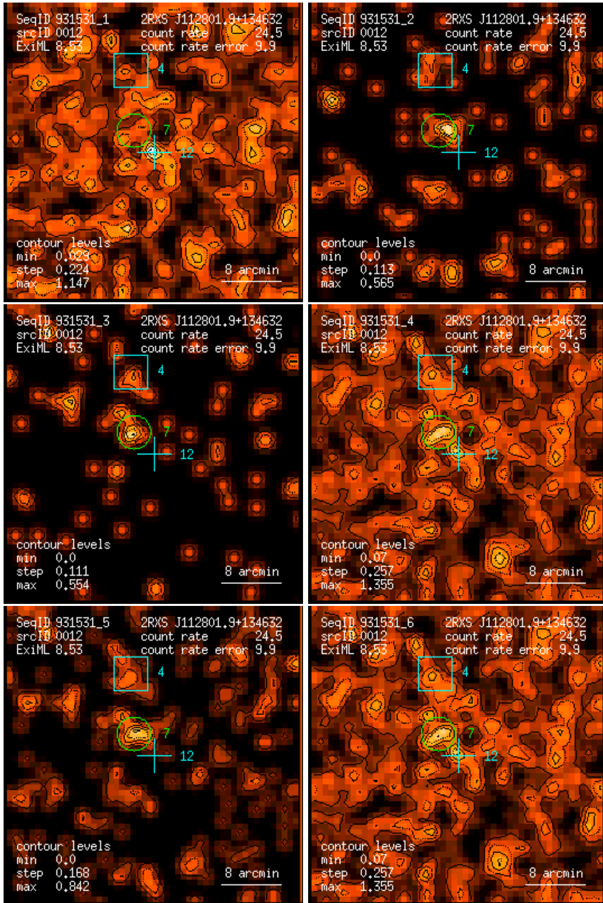
Figure 12: RASS 931531: detection 0012: band rate images, Gaussian filter: (1) PSPC channels 11 – 41, (2) 52 – 90, (3) 91 – 201, (4) 11 – 235, (5) 52 – 201, (6) 11 – 201. Broad band rates in counts/ks. Band rate contour levels in counts/ks/arcmin 2 .
