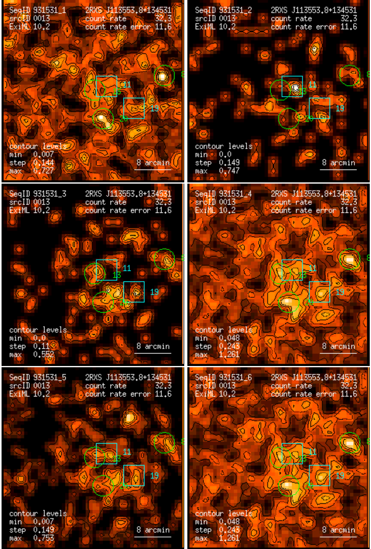
Figure 13: RASS 931531: detection 0013: band rate images, Gaussian filter: (1) PSPC channels 11 – 41, (2) 52 – 90, (3) 91 – 201, (4) 11 – 235, (5) 52 – 201, (6) 11 – 201. Broad band rates in counts/ks. Band rate contour levels in counts/ks/arcmin 2 .
