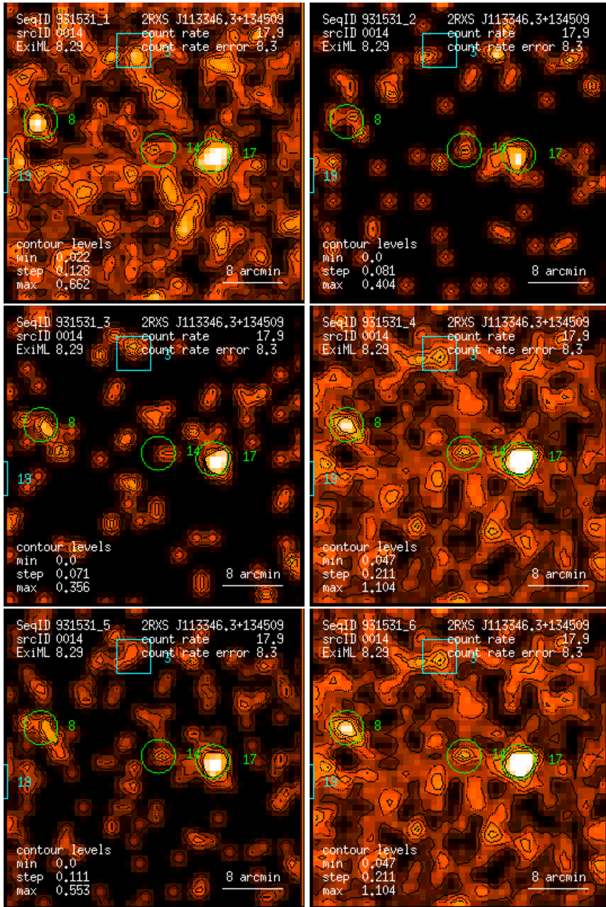
Figure 14: RASS 931531: detection 0014: band rate images, Gaussian filter: (1) PSPC channels 11 – 41, (2) 52 – 90, (3) 91 – 201, (4) 11 – 235, (5) 52 – 201, (6) 11 – 201. Broad band rates in counts/ks. Band rate contour levels in counts/ks/arcmin 2 .
