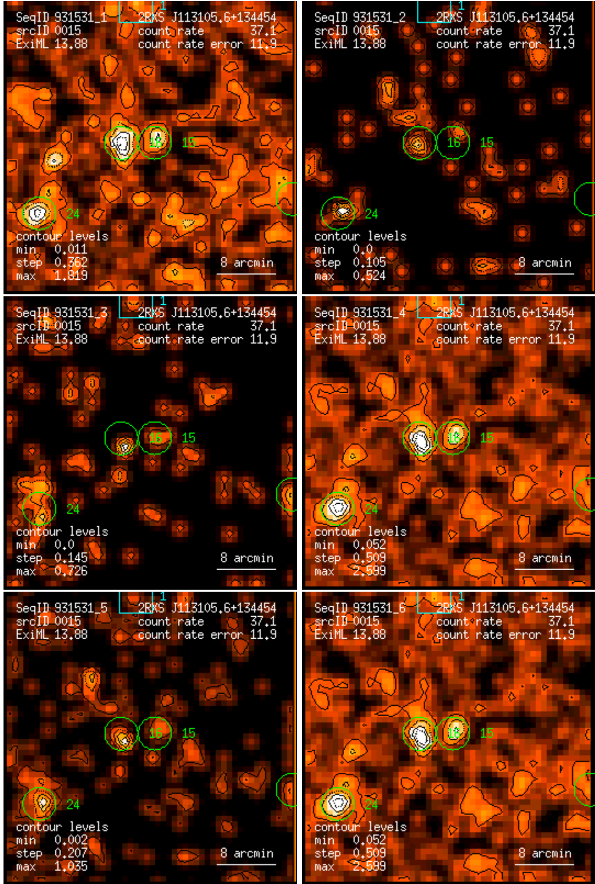
Figure 15: RASS 931531: detection 0015: band rate images, Gaussian filter: (1) PSPC channels 11 – 41, (2) 52 – 90, (3) 91 – 201, (4) 11 – 235, (5) 52 – 201, (6) 11 – 201. Broad band rates in counts/ks. Band rate contour levels in counts/ks/arcmin 2 .
