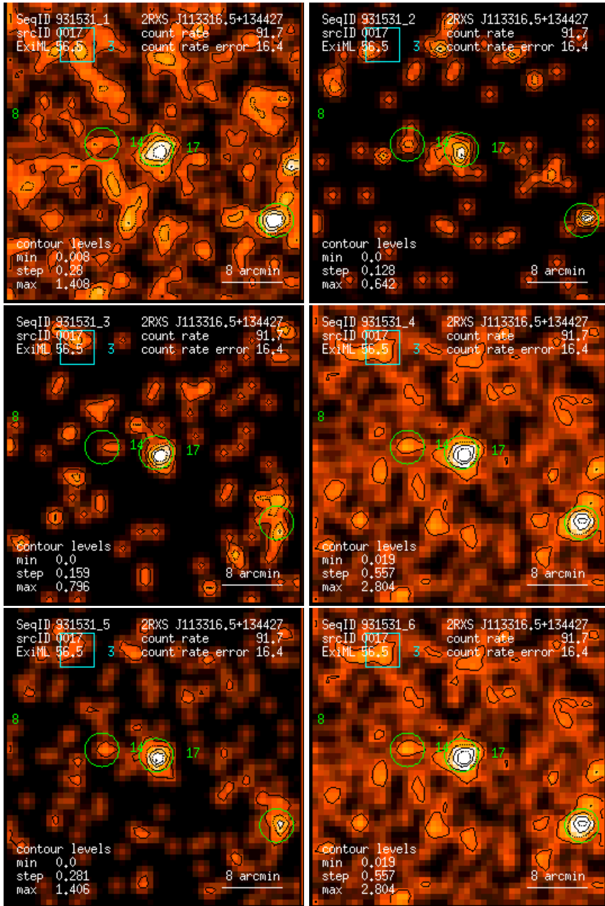
Figure 17: RASS 931531: detection 0017: band rate images, Gaussian filter: (1) PSPC channels 11 – 41, (2) 52 – 90, (3) 91 – 201, (4) 11 – 235, (5) 52 – 201, (6) 11 – 201. Broad band rates in counts/ks. Band rate contour levels in counts/ks/arcmin 2 .
