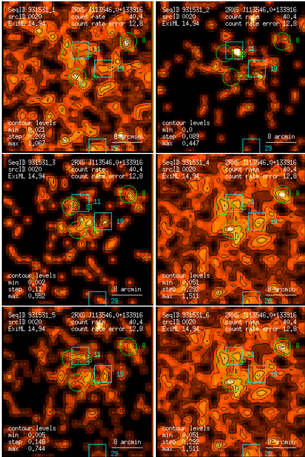
Figure 20: RASS 931531: detection 0020: band rate images, Gaussian filter: (1) PSPC channels 11 – 41, (2) 52 – 90, (3) 91 – 201, (4) 11 – 235, (5) 52 – 201, (6) 11 – 201. Broad band rates in counts/ks. Band rate contour levels in counts/ks/arcmin 2 .
