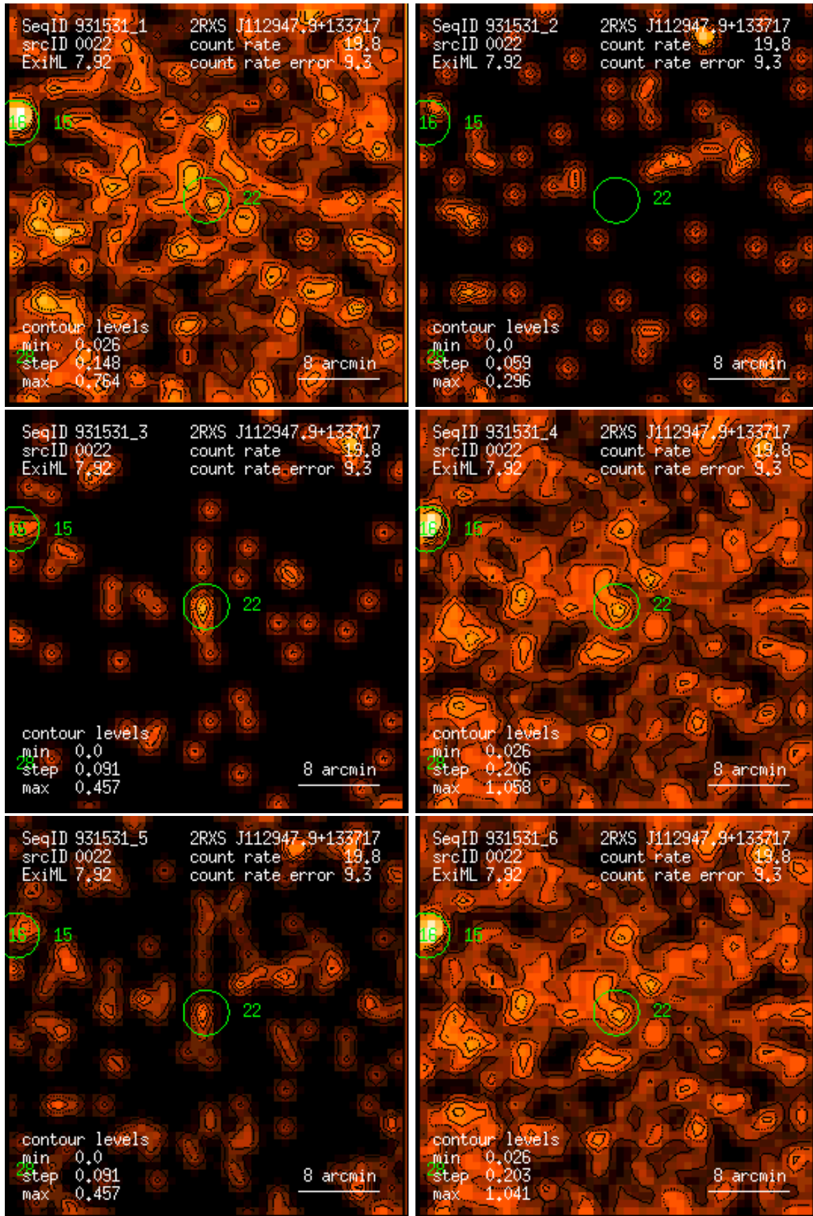
Figure 22: RASS 931531: detection 0022: band rate images, Gaussian filter: (1) PSPC channels 11 – 41, (2) 52 – 90, (3) 91 – 201, (4) 11 – 235, (5) 52 – 201, (6) 11 – 201. Broad band rates in counts/ks. Band rate contour levels in counts/ks/arcmin 2 .
