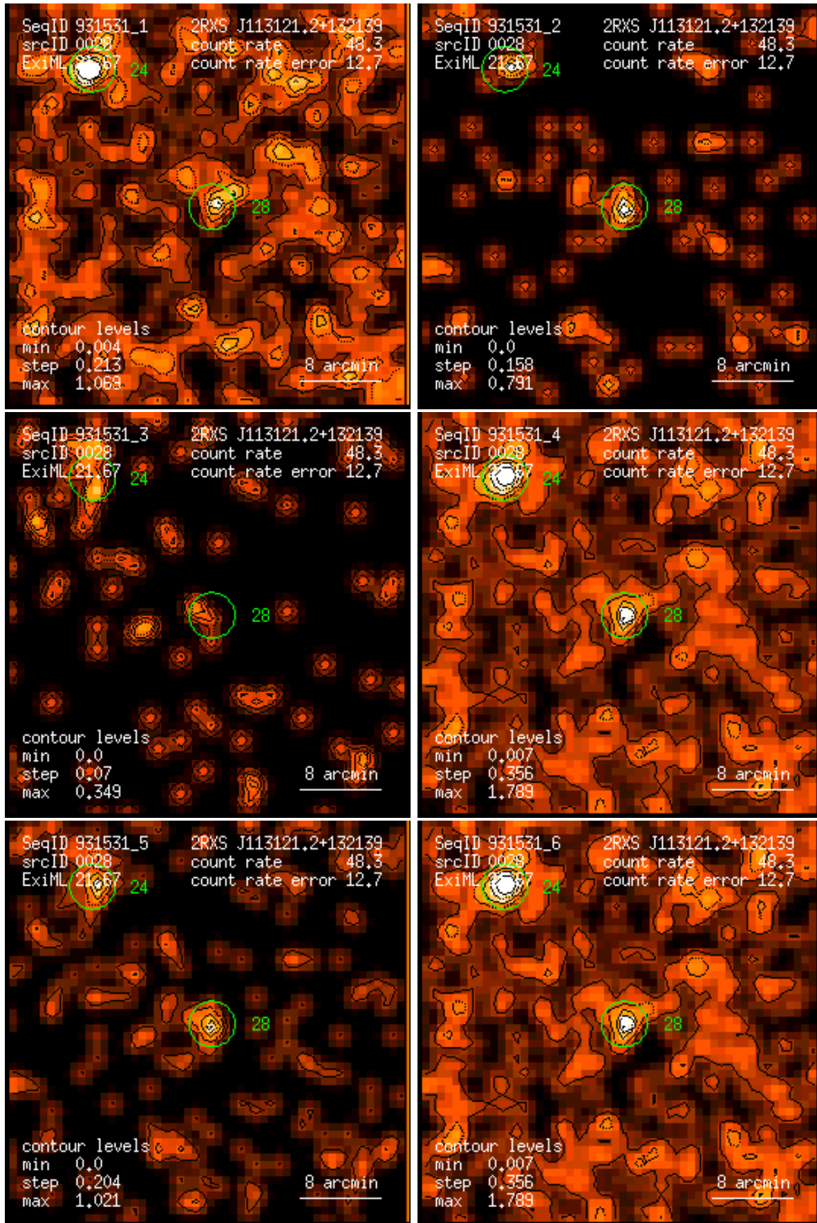
Figure 28: RASS 931531: detection 0028: band rate images, Gaussian filter: (1) PSPC channels 11 – 41, (2) 52 – 90, (3) 91 – 201, (4) 11 – 235, (5) 52 – 201, (6) 11 – 201. Broad band rates in counts/ks. Band rate contour levels in counts/ks/arcmin 2 .
