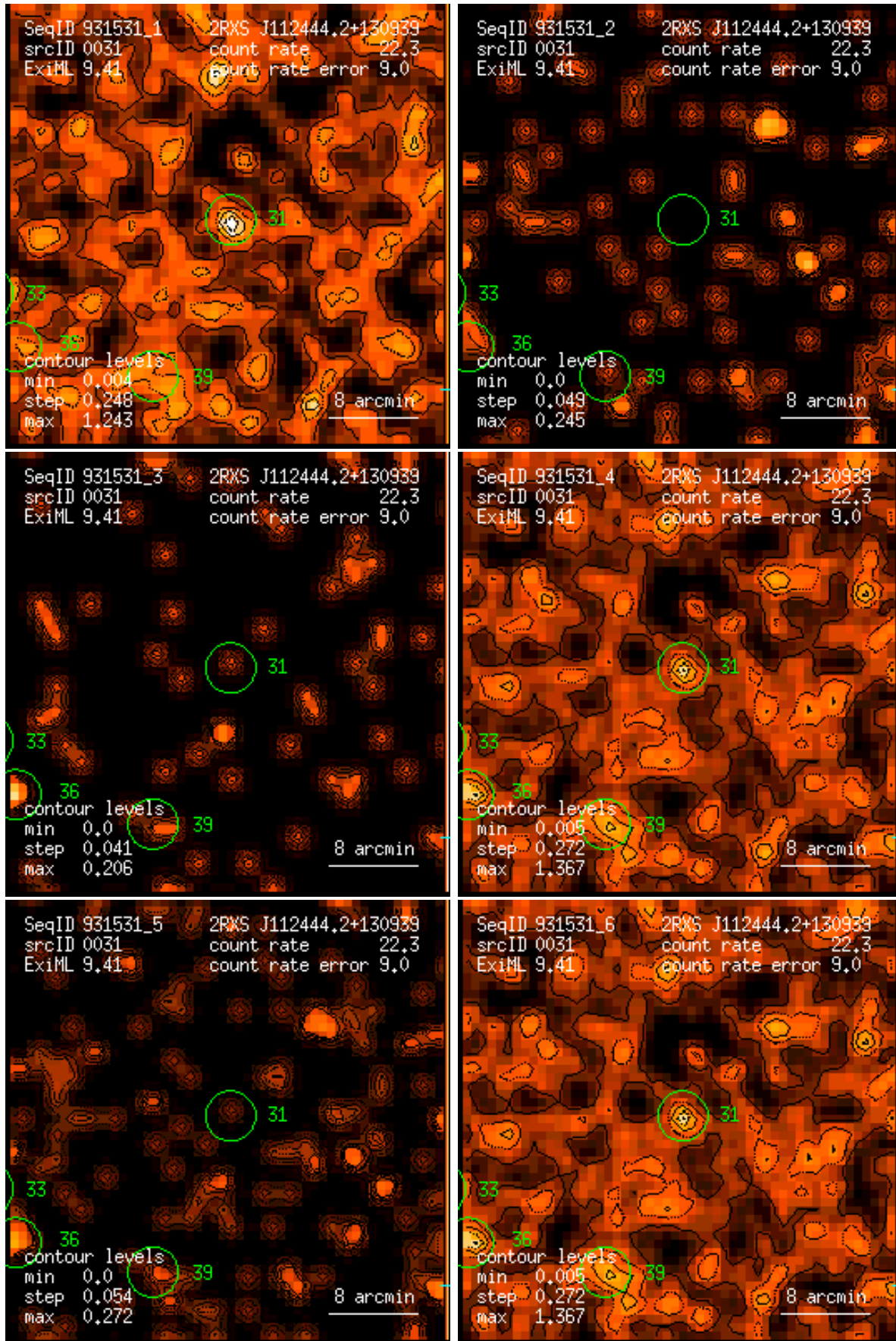
Figure 31: RASS 931531: detection 0031: band rate images, Gaussian filter: (1) PSPC channels 11 – 41, (2) 52 – 90, (3) 91 – 201, (4) 11 – 235, (5) 52 – 201, (6) 11 – 201. Broad band rates in counts/ks. Band rate contour levels in counts/ks/arcmin 2 .
