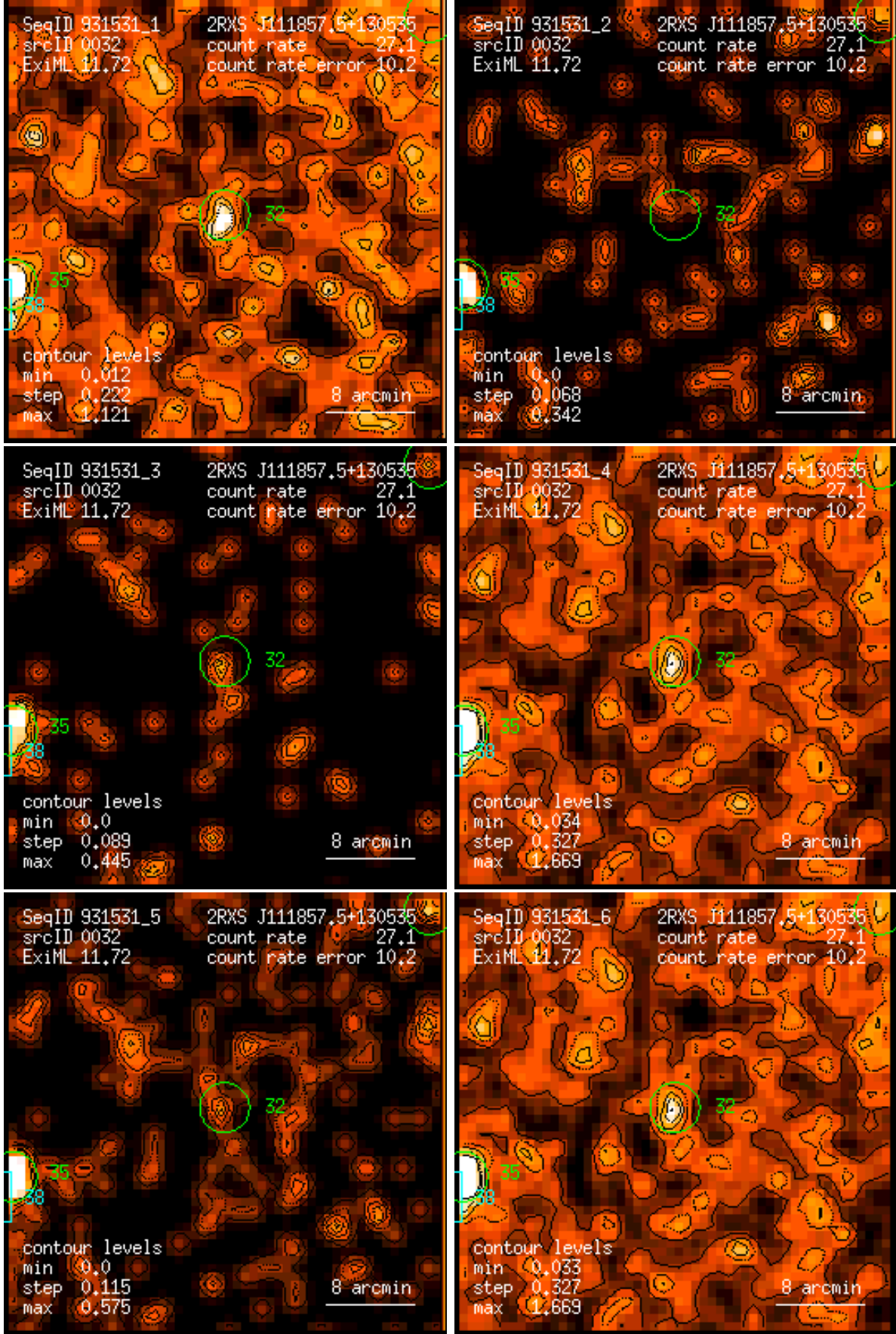
Figure 32: RASS 931531: detection 0032: band rate images, Gaussian filter: (1) PSPC channels 11 – 41, (2) 52 – 90, (3) 91 – 201, (4) 11 – 235, (5) 52 – 201, (6) 11 – 201. Broad band rates in counts/ks. Band rate contour levels in counts/ks/arcmin 2 .
