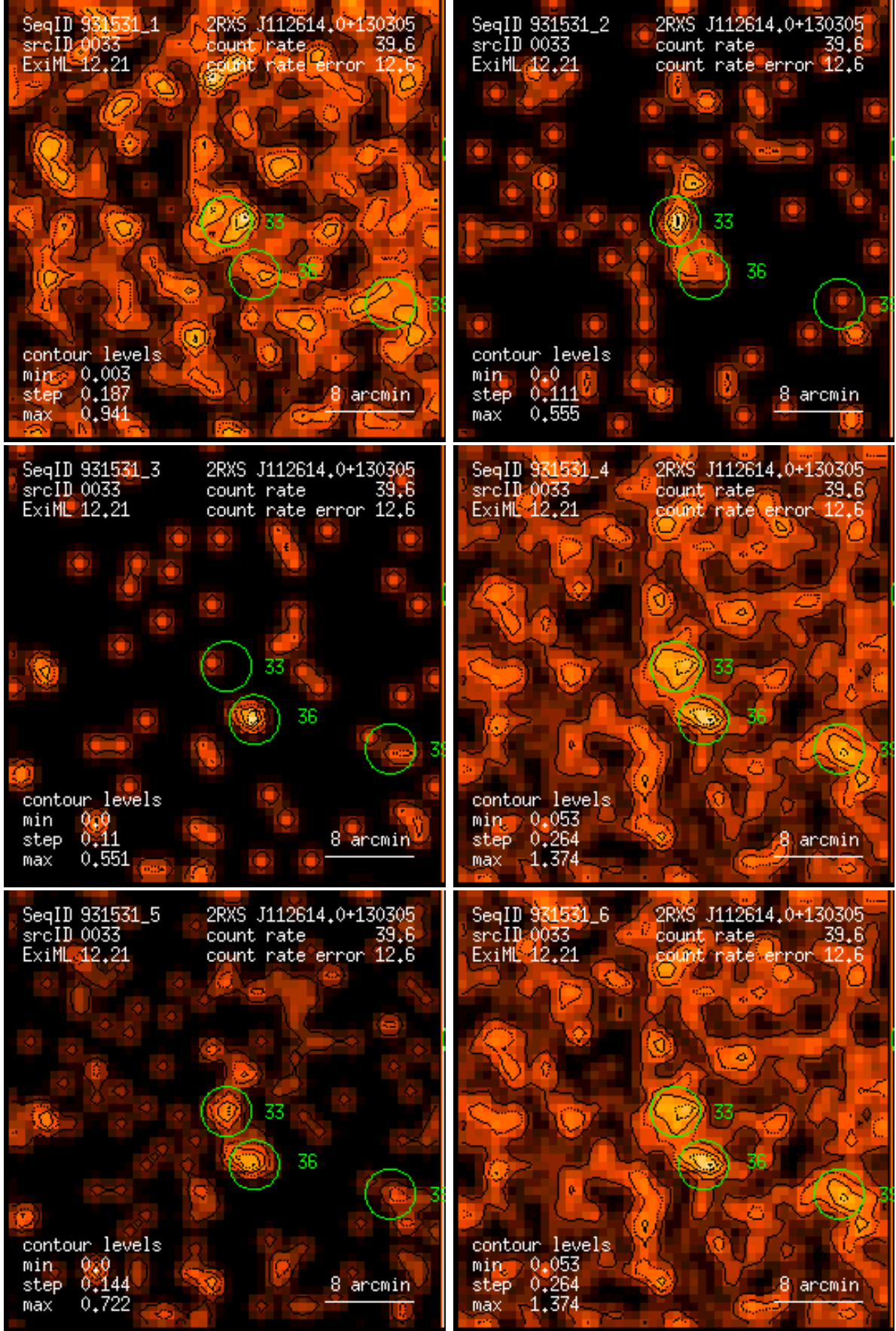
Figure 33: RASS 931531: detection 0033: band rate images, Gaussian filter: (1) PSPC channels 11 – 41, (2) 52 – 90, (3) 91 – 201, (4) 11 – 235, (5) 52 – 201, (6) 11 – 201. Broad band rates in counts/ks. Band rate contour levels in counts/ks/arcmin 2 .
