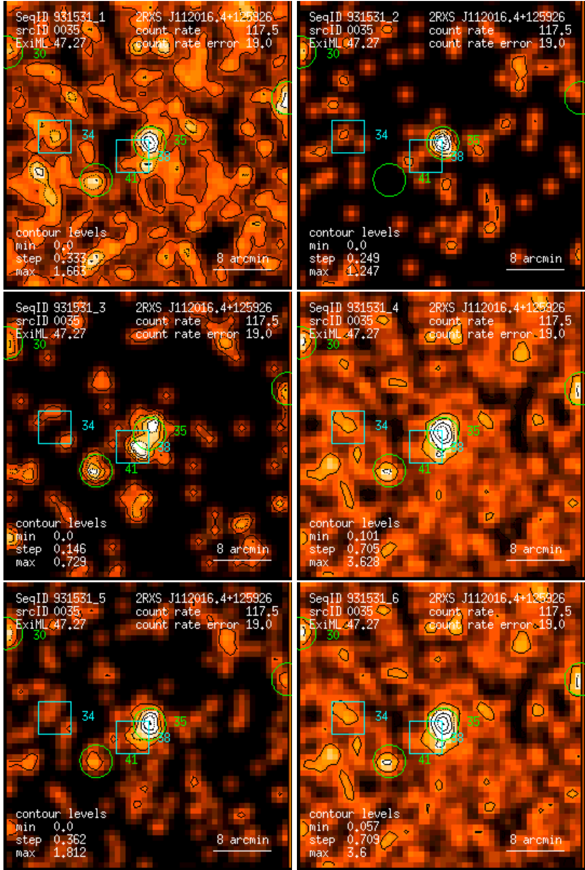
Figure 35: RASS 931531: detection 0035: band rate images, Gaussian filter: (1) PSPC channels 11 – 41, (2) 52 – 90, (3) 91 – 201, (4) 11 – 235, (5) 52 – 201, (6) 11 – 201. Broad band rates in counts/ks. Band rate contour levels in counts/ks/arcmin 2 .
