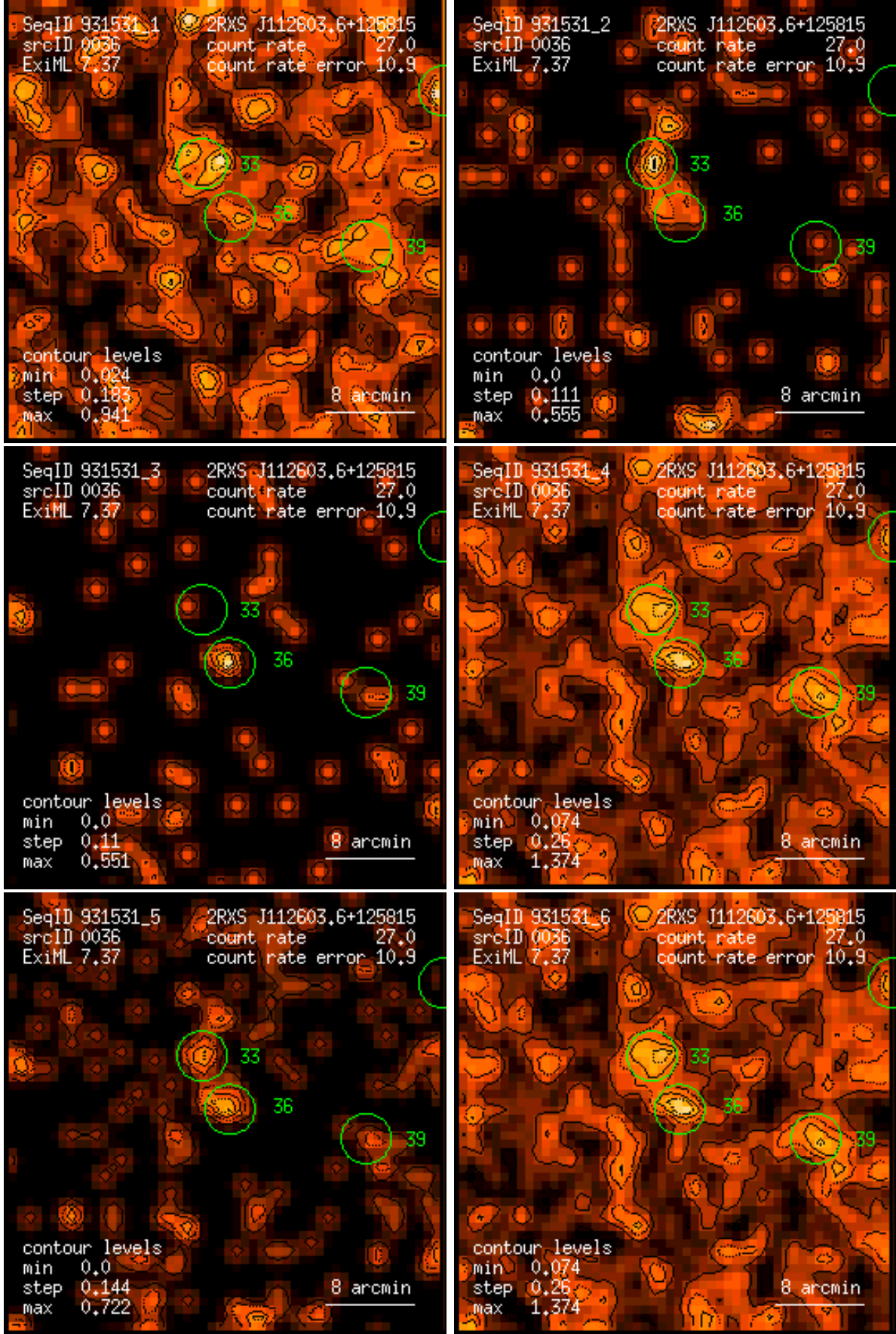
Figure 36: RASS 931531: detection 0036: band rate images, Gaussian filter: (1) PSPP channels 11 – 41, (2) 52 – 90, (3) 91 – 201, (4) 11 – 235, (5) 52 – 201, (6) 11 – 201. Broad band rates in counts/ks. Band rate contour levels in counts/ks/arcmin 2 .
