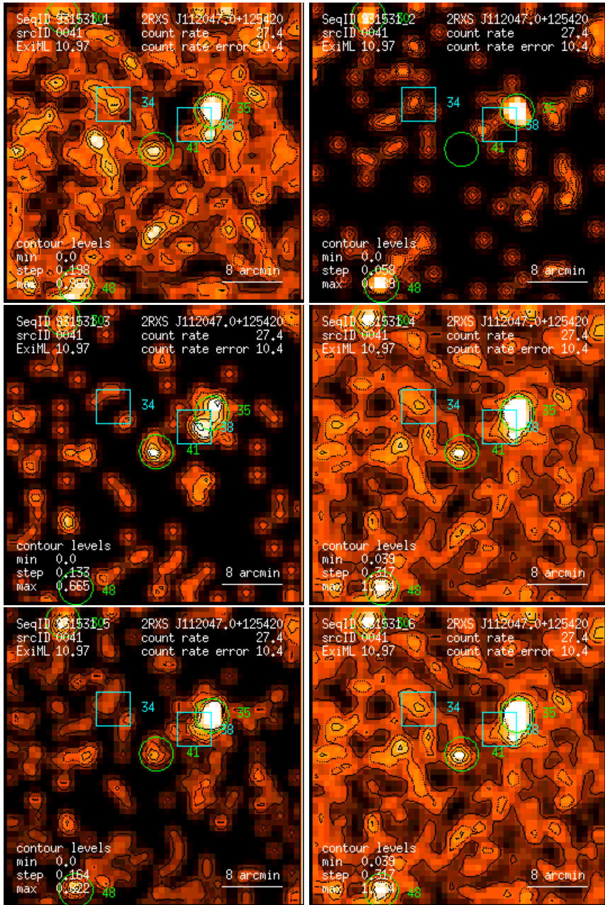
Figure 41: RASS 931531: detection 0041: band rate images, Gaussian filter: (1) PSPC channels 11 – 41, (2) 52 – 90, (3) 91 – 201, (4) 11 – 235, (5) 52 – 201, (6) 11 – 201. Broad band rates in counts/ks. Band rate contour levels in counts/ks/arcmin 2 .
