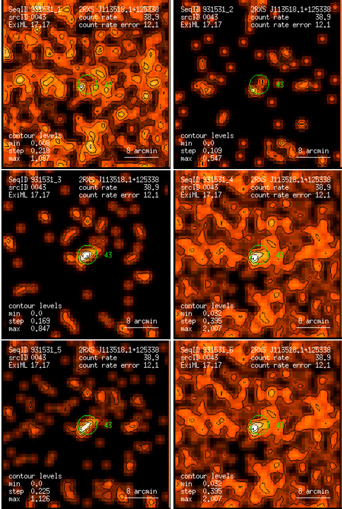
Figure 43: RASS 931531: detection 0043: band rate images, Gaussian filter: (1) PSPC channels 11 – 41, (2) 52 – 90, (3) 91 – 201, (4) 11 – 235, (5) 52 – 201, (6) 11 – 201. Broad band rates in counts/ks. Band rate contour levels in counts/ks/arcmin 2 .
