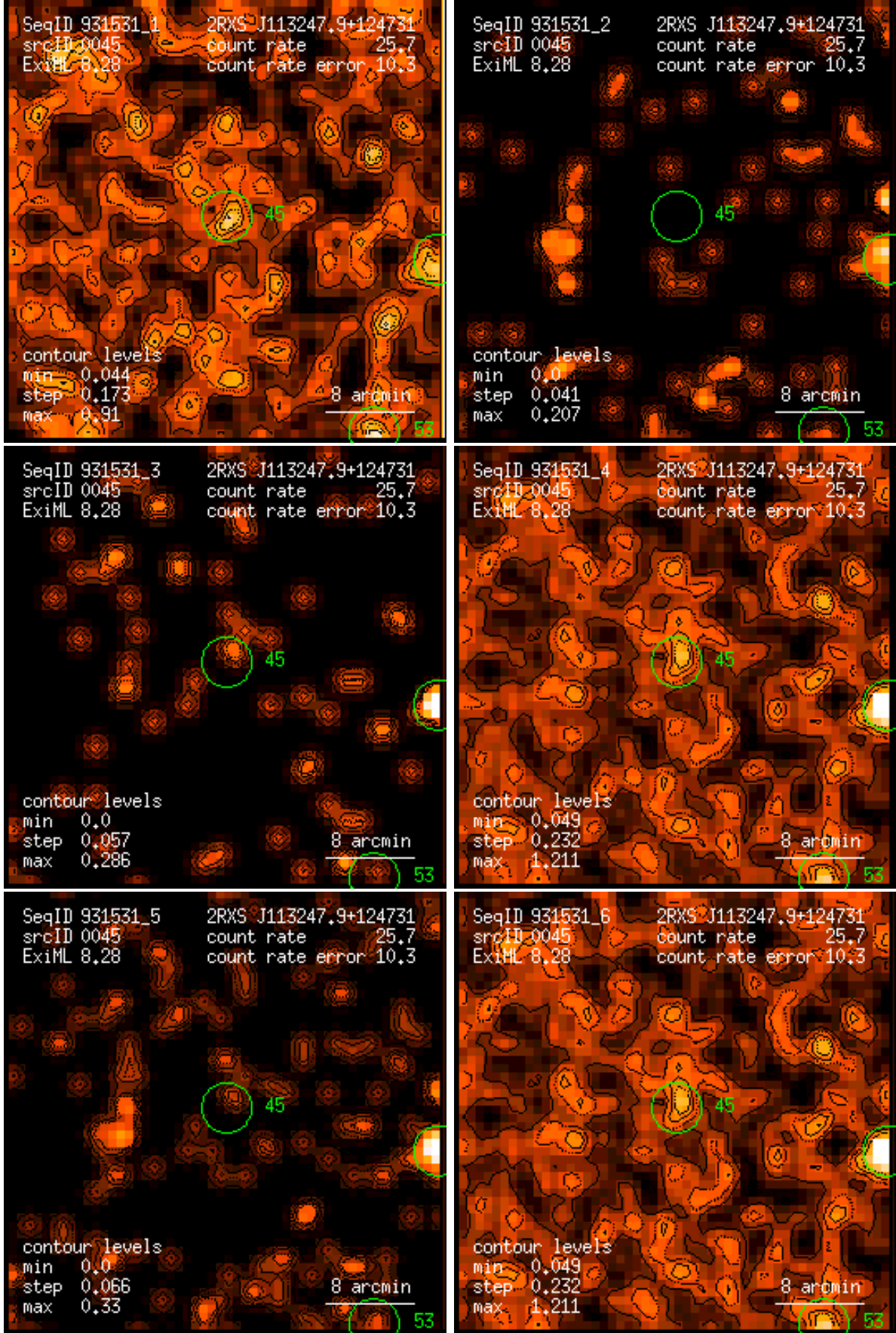
Figure 45: RASS 931531: detection 0045: band rate images, Gaussian filter: (1) PSPC channels 11 – 41, (2) 52 – 90, (3) 91 – 201, (4) 11 – 235, (5) 52 – 201, (6) 11 – 201. Broad band rates in counts/ks. Band rate contour levels in counts/ks/arcmin 2 .
