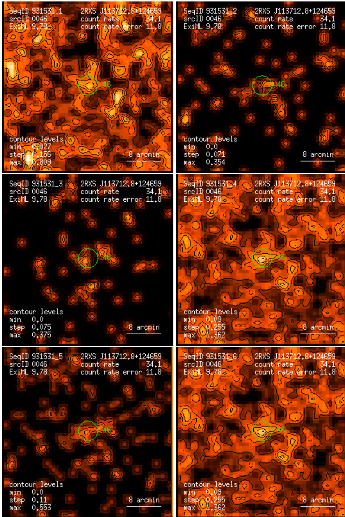
Figure 46: RASS 931531: detection 0046: band rate images, Gaussian filter: (1) PSPC channels 11 – 41, (2) 52 – 90, (3) 91 – 201, (4) 11 – 235, (5) 52 – 201, (6) 11 – 201. Broad band rates in counts/ks. Band rate contour levels in counts/ks/arcmin 2 .
