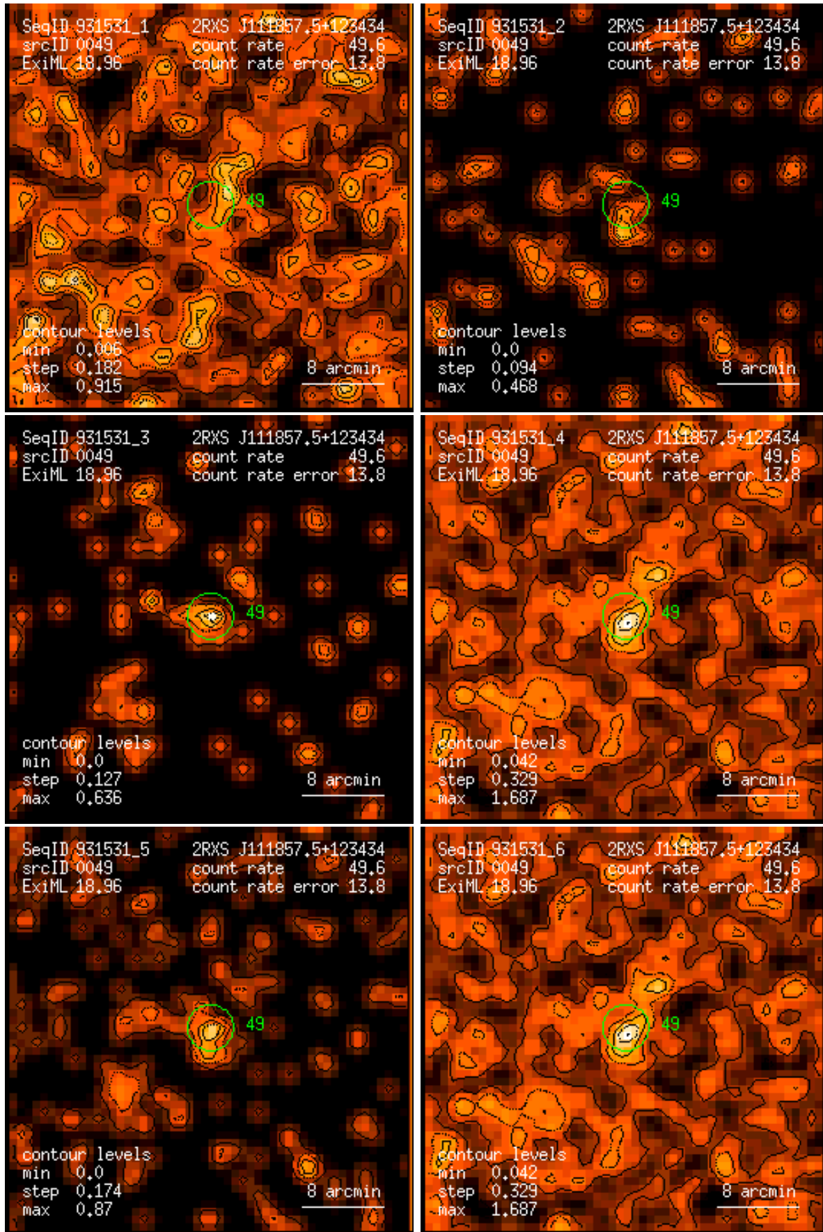
Figure 49: RASS 931531: detection 0049: band rate images, Gaussian filter: (1) PSPC channels 11 – 41, (2) 52 – 90, (3) 91 – 201, (4) 11 – 235, (5) 52 – 201, (6) 11 – 201. Broad band rates in counts/ks. Band rate contour levels in counts/ks/arcmin 2 .
