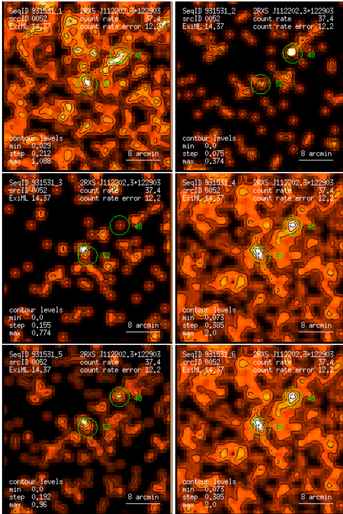
Figure 52: RASS 931531: detection 0052: band rate images, Gaussian filter: (1) PSPC channels 11 – 41, (2) 52 – 90, (3) 91 – 201, (4) 11 – 235, (5) 52 – 201, (6) 11 – 201. Broad band rates in counts/ks. Band rate contour levels in counts/ks/arcmin 2 .
