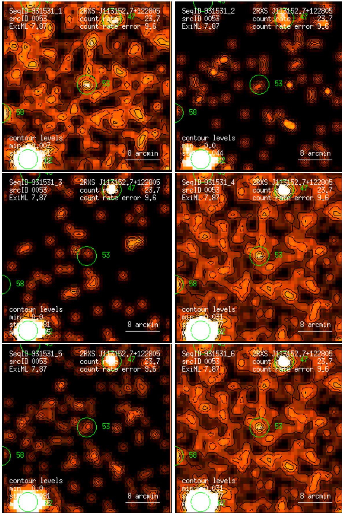
Figure 53: RASS 931531: detection 0053: band rate images, Gaussian filter: (1) PSPC channels 11 – 41, (2) 52 – 90, (3) 91 – 201, (4) 11 – 235, (5) 52 – 201, (6) 11 – 201. Broad band rates in counts/ks. Band rate contour levels in counts/ks/arcmin 2 .
