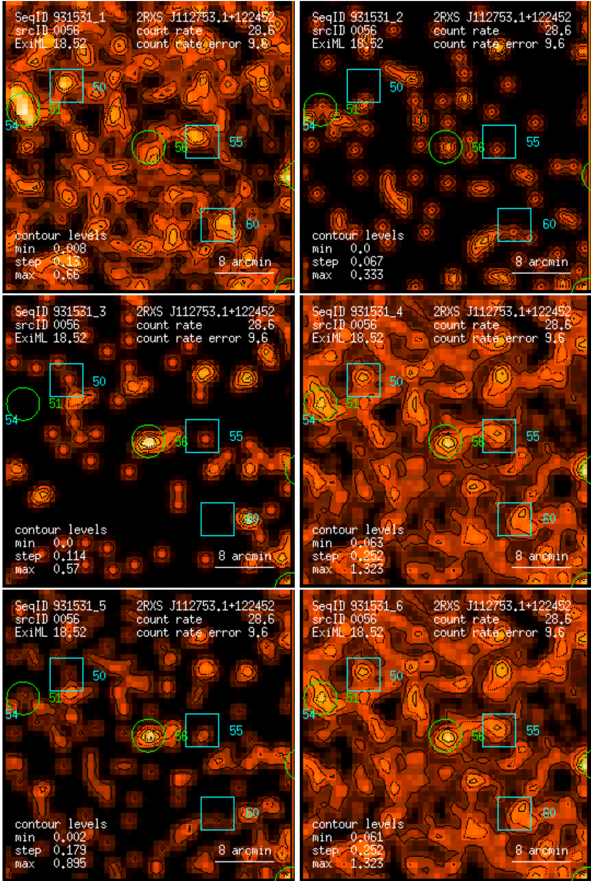
Figure 56: RASS 931531: detection 0056: band rate images, Gaussian filter: (1) PSPC channels 11 – 41, (2) 52 – 90, (3) 91 – 201, (4) 11 – 235, (5) 52 – 201, (6) 11 – 201. Broad band rates in counts/ks. Band rate contour levels in counts/ks/arcmin 2 .
