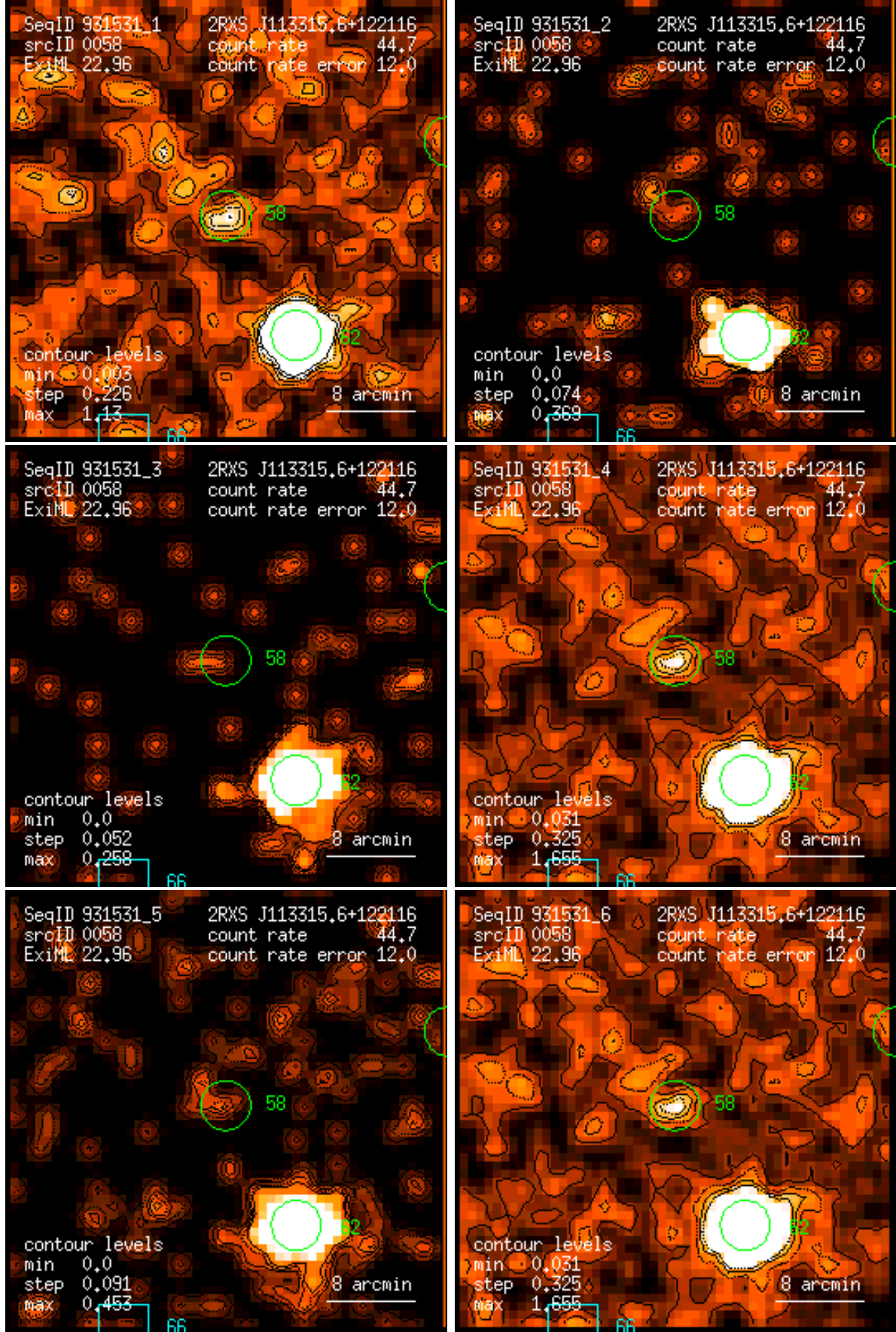
Figure 58: RASS 931531: detection 0058: band rate images, Gaussian filter: (1) PSPC channels 11 – 41, (2) 52 – 90, (3) 91 – 201, (4) 11 – 235, (5) 52 – 201, (6) 11 – 201. Broad band rates in counts/ks. Band rate contour levels in counts/ks/arcmin 2 .
