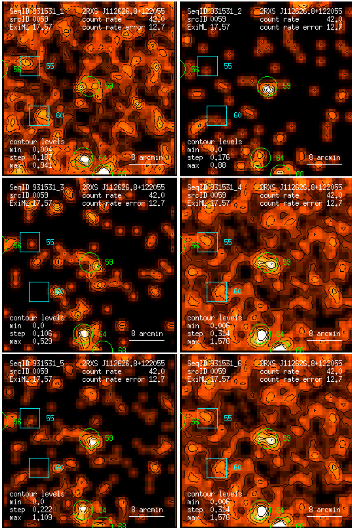
Figure 59: RASS 931531: detection 0059: band rate images, Gaussian filter: (1) PSPC channels 11 – 41, (2) 52 – 90, (3) 91 – 201, (4) 11 – 235, (5) 52 – 201, (6) 11 – 201. Broad band rates in counts/ks. Band rate contour levels in counts/ks/arcmin 2 .
