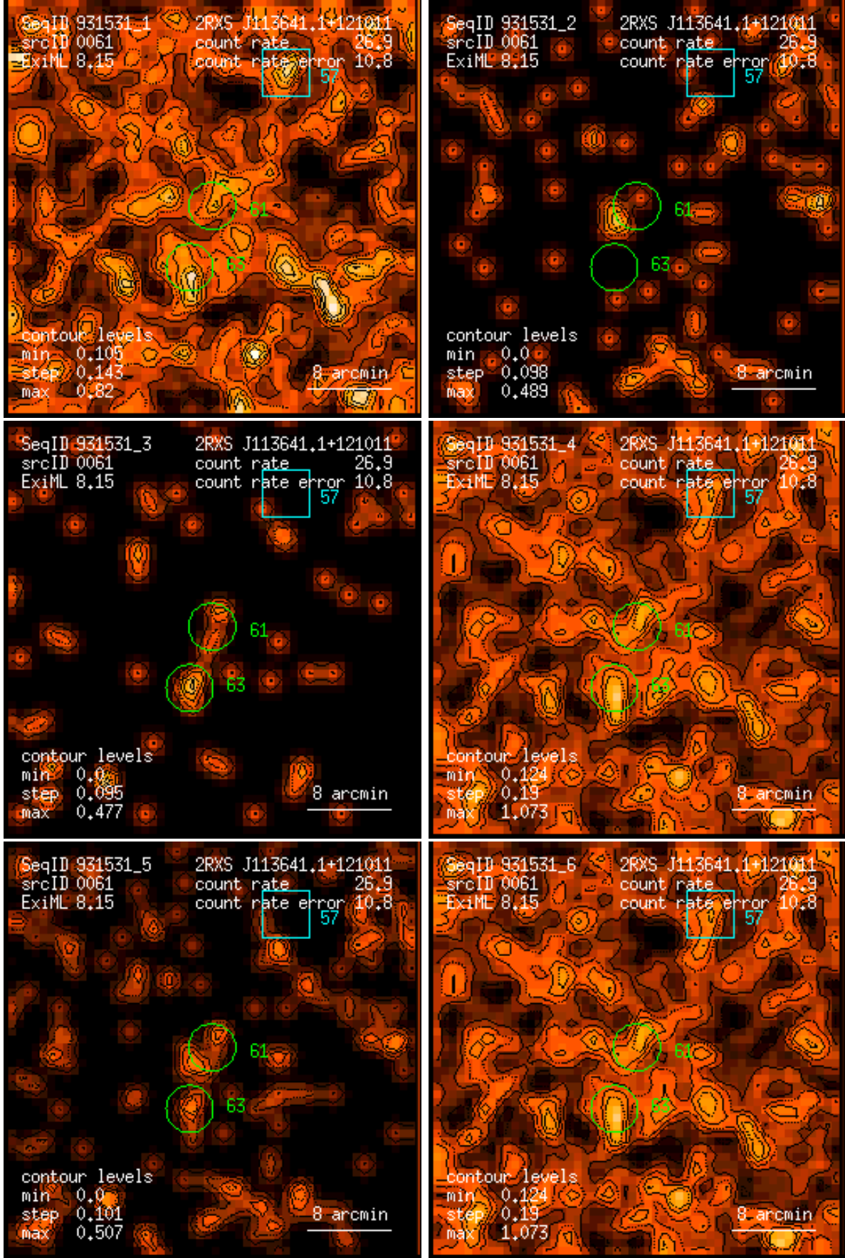
Figure 61: RASS 931531: detection 0061: band rate images, Gaussian filter: (1) PSPC channels 11 – 41, (2) 52 – 90, (3) 91 – 201, (4) 11 – 235, (5) 52 – 201, (6) 11 – 201. Broad band rates in counts/ks. Band rate contour levels in counts/ks/arcmin 2 .
