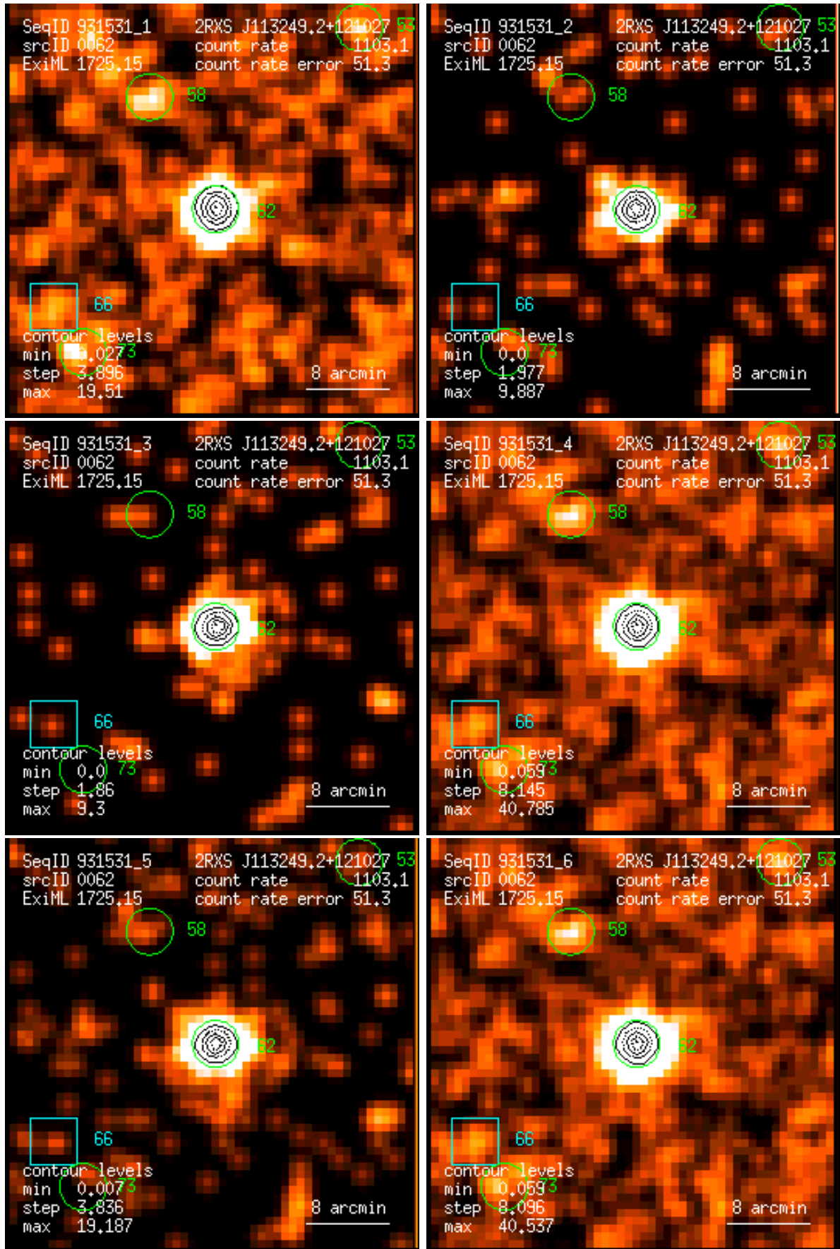
Figure 62: RASS 931531: detection 0062: band rate images, Gaussian filter: (1) PSPC channels 11 – 41, (2) 52 – 90, (3) 91 – 201, (4) 11 – 235, (5) 52 – 201, (6) 11 – 201. Broad band rates in counts/ks. Band rate contour levels in counts/ks/arcmin 2 .
