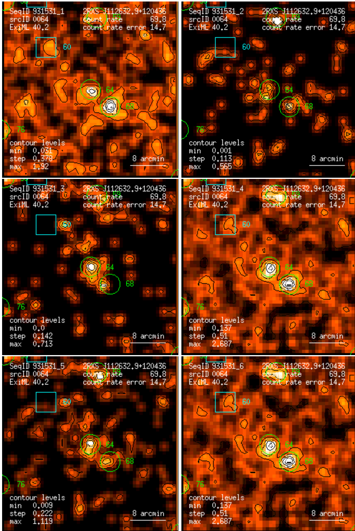
Figure 64: RASS 931531: detection 0064: band rate images, Gaussian filter: (1) PSPC channels 11 – 41, (2) 52 – 90, (3) 91 – 201, (4) 11 – 235, (5) 52 – 201, (6) 11 – 201. Broad band rates in counts/ks. Band rate contour levels in counts/ks/arcmin 2 .
