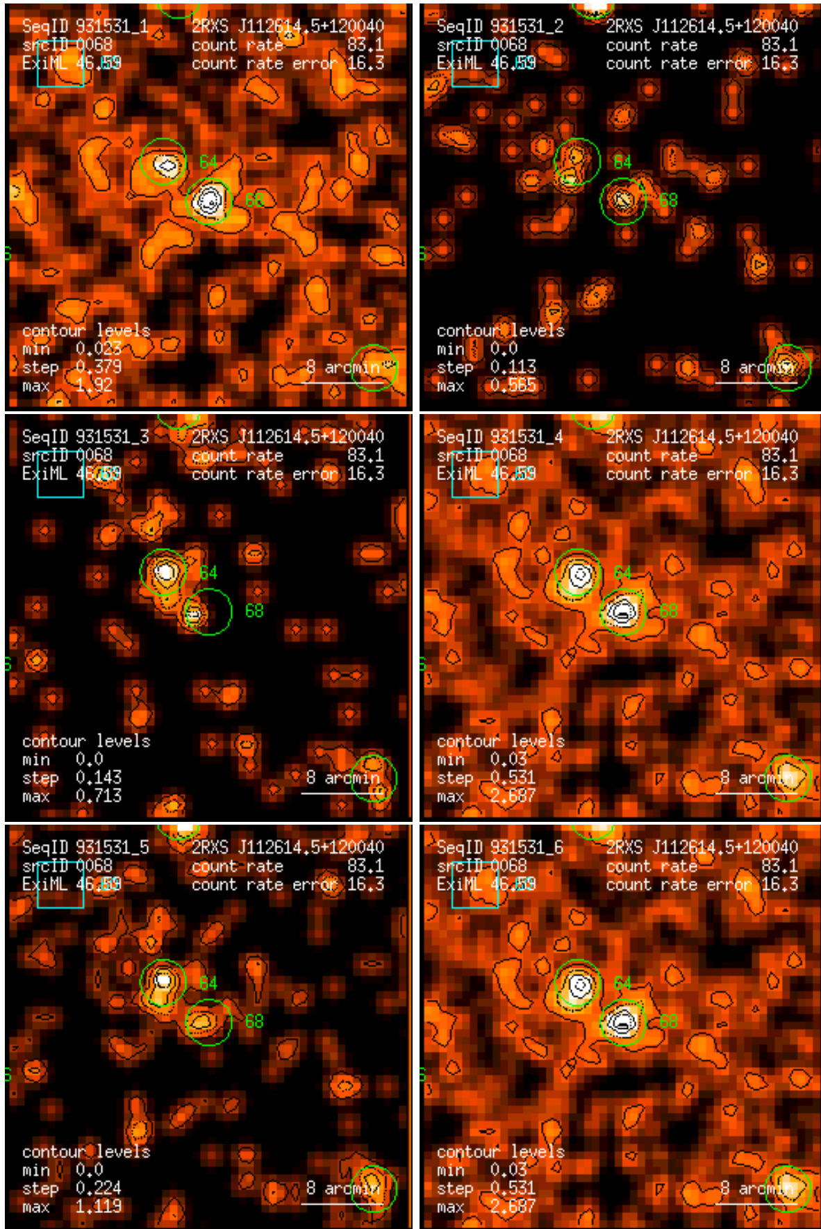
Figure 68: RASS 931531: detection 0068: band rate images, Gaussian filter: (1) PSPC channels 11 – 41, (2) 52 – 90, (3) 91 – 201, (4) 11 – 235, (5) 52 – 201, (6) 11 – 201. Broad band rates in counts/ks. Band rate contour levels in counts/ks/arcmin 2 .
