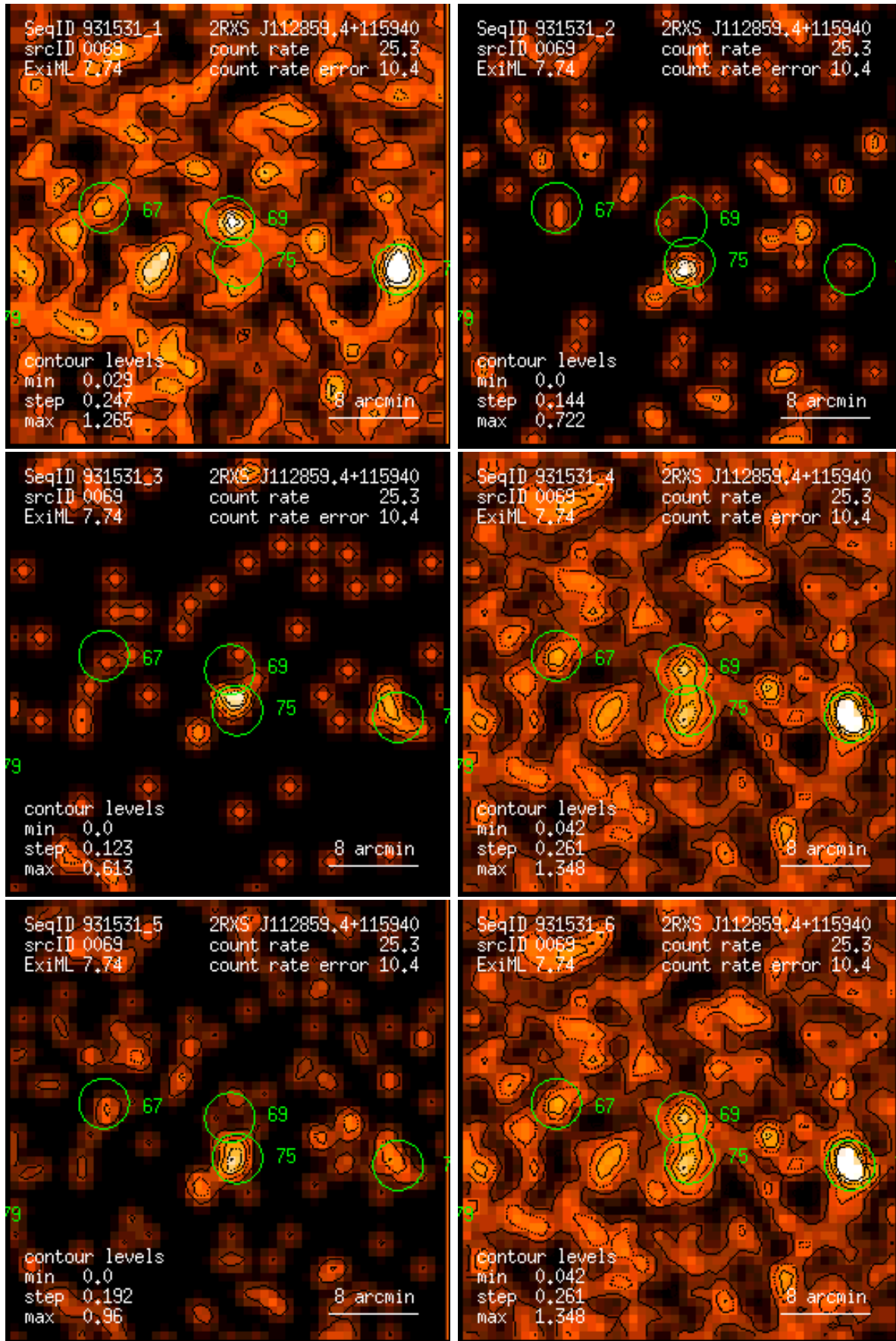
Figure 69: RASS 931531: detection 0069: band rate images, Gaussian filter: (1) PSPC channels 11 – 41, (2) 52 – 90, (3) 91 – 201, (4) 11 – 235, (5) 52 – 201, (6) 11 – 201. Broad band rates in counts/ks. Band rate contour levels in counts/ks/arcmin 2 .
