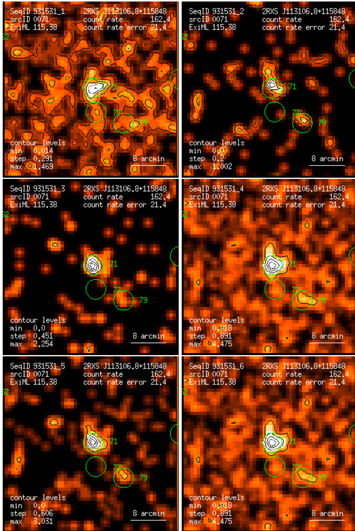
Figure 71: RASS 931531: detection 0071: band rate images, Gaussian filter: (1) PSPC channels 11 – 41, (2) 52 – 90, (3) 91 – 201, (4) 11 – 235, (5) 52 – 201, (6) 11 – 201. Broad band rates in counts/ks. Band rate contour levels in counts/ks/arcmin 2 .
