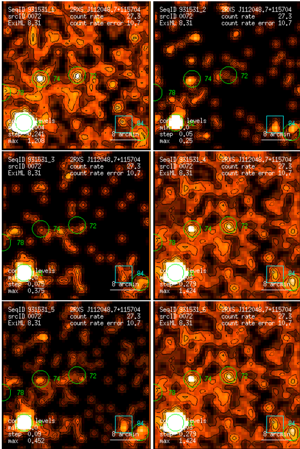
Figure 72: RASS 931531: detection 0072: band rate images, Gaussian filter: (1) PSPC channels 11 – 41, (2) 52 – 90, (3) 91 – 201, (4) 11 – 235, (5) 52 – 201, (6) 11 – 201. Broad band rates in counts/ks. Band rate contour levels in counts/ks/arcmin 2 .
