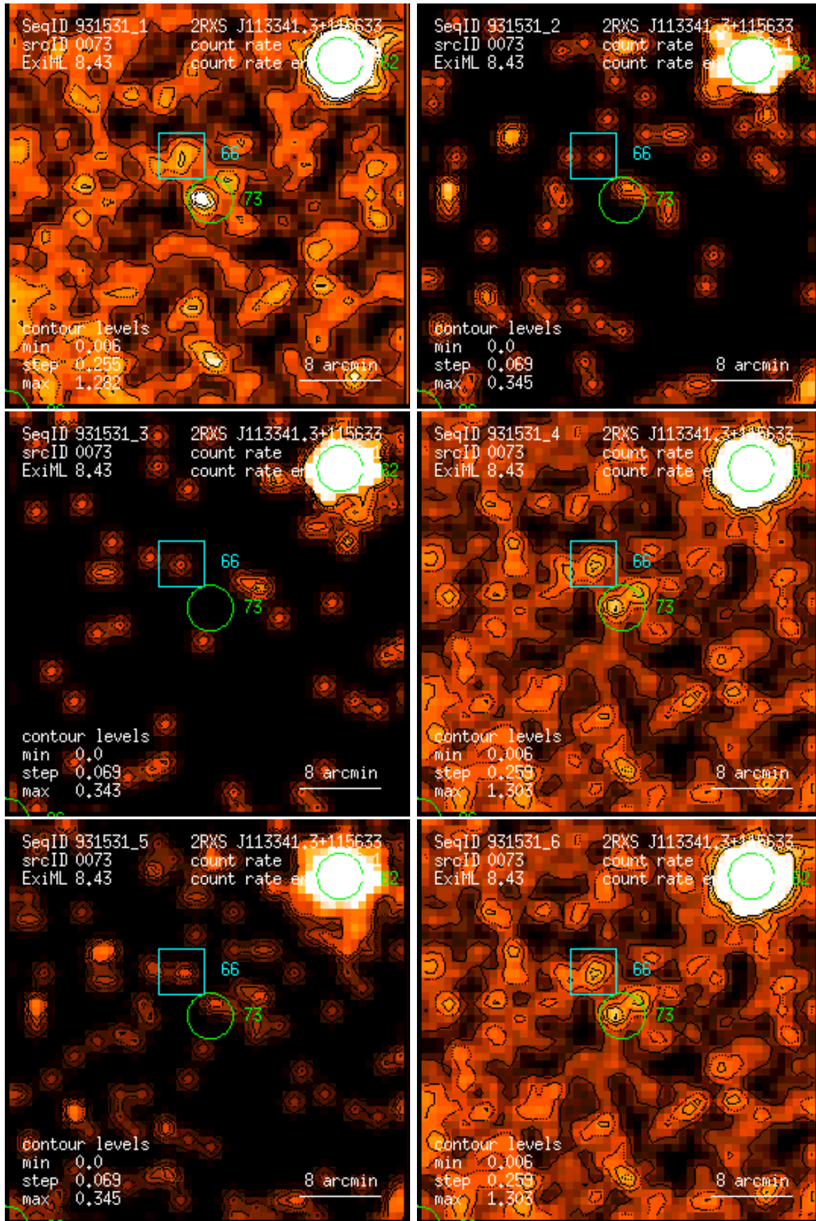
Figure 73: RASS 931531: detection 0073: band rate images, Gaussian filter: (1) PSPC channels 11 – 41, (2) 52 – 90, (3) 91 – 201, (4) 11 – 235, (5) 52 – 201, (6) 11 – 201. Broad band rates in counts/ks. Band rate contour levels in counts/ks/arcmin 2 .
