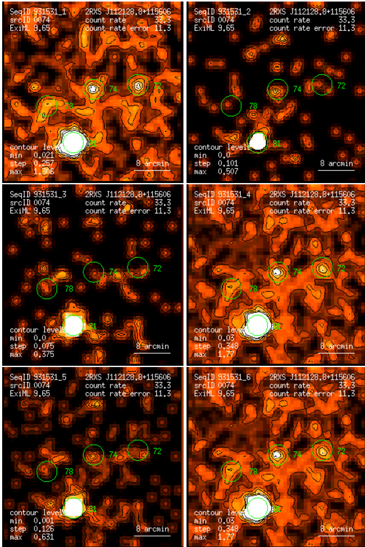
Figure 74: RASS 931531: detection 0074: band rate images, Gaussian filter: (1) PSPC channels 11 – 41, (2) 52 – 90, (3) 91 – 201, (4) 11 – 235, (5) 52 – 201, (6) 11 – 201. Broad band rates in counts/ks. Band rate contour levels in counts/ks/arcmin 2 .
