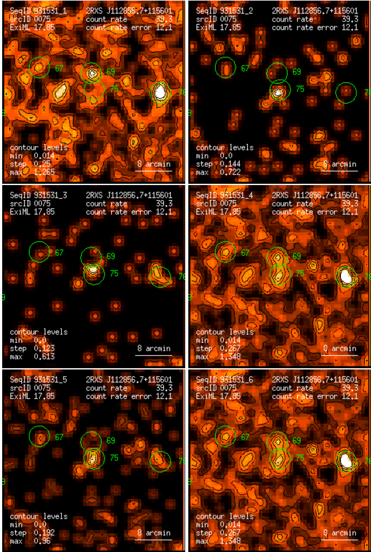
Figure 75: RASS 931531: detection 0075: band rate images, Gaussian filter: (1) PSPC channels 11 – 41, (2) 52 – 90, (3) 91 – 201, (4) 11 – 235, (5) 52 – 201, (6) 11 – 201. Broad band rates in counts/ks. Band rate contour levels in counts/ks/arcmin 2 .
